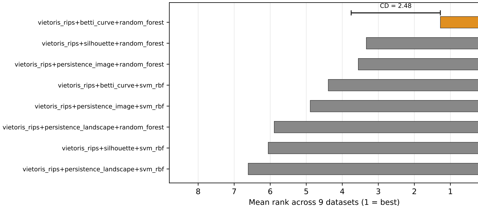
Nemenyi critical difference: config mean ranks across 9 datasets
