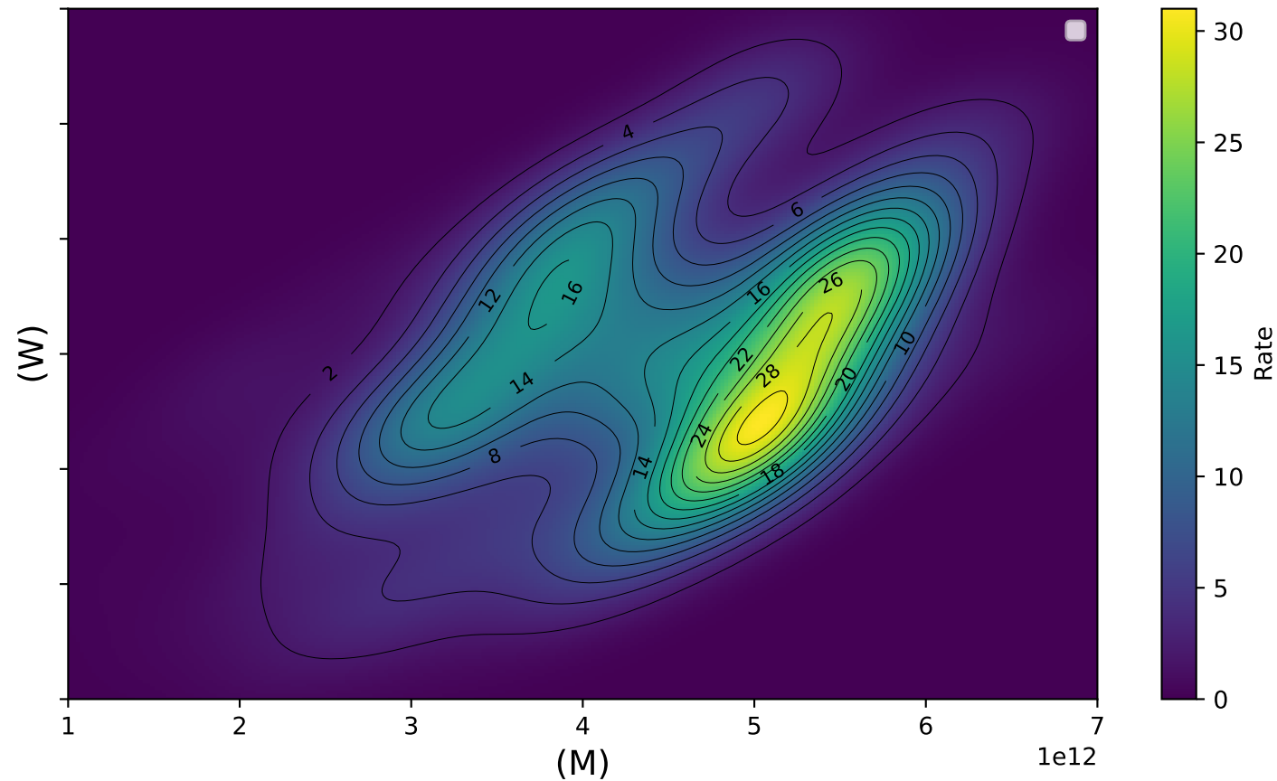
Rate of the Poisson Process
