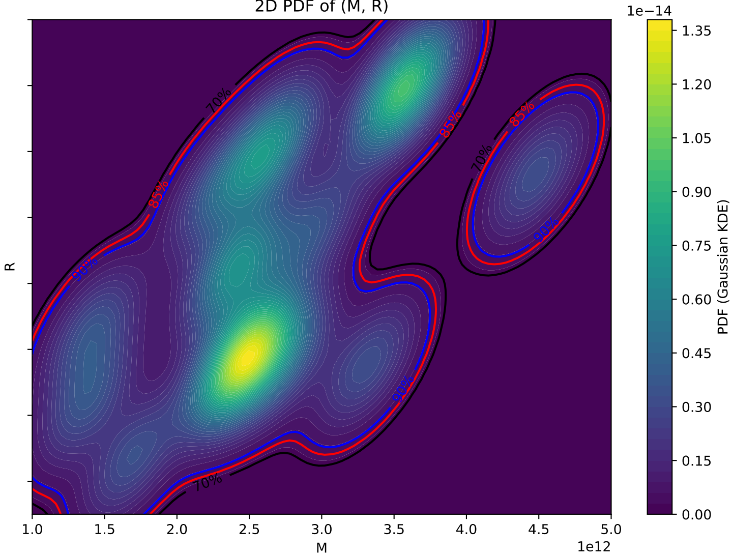
2D PDF of (M, R)
