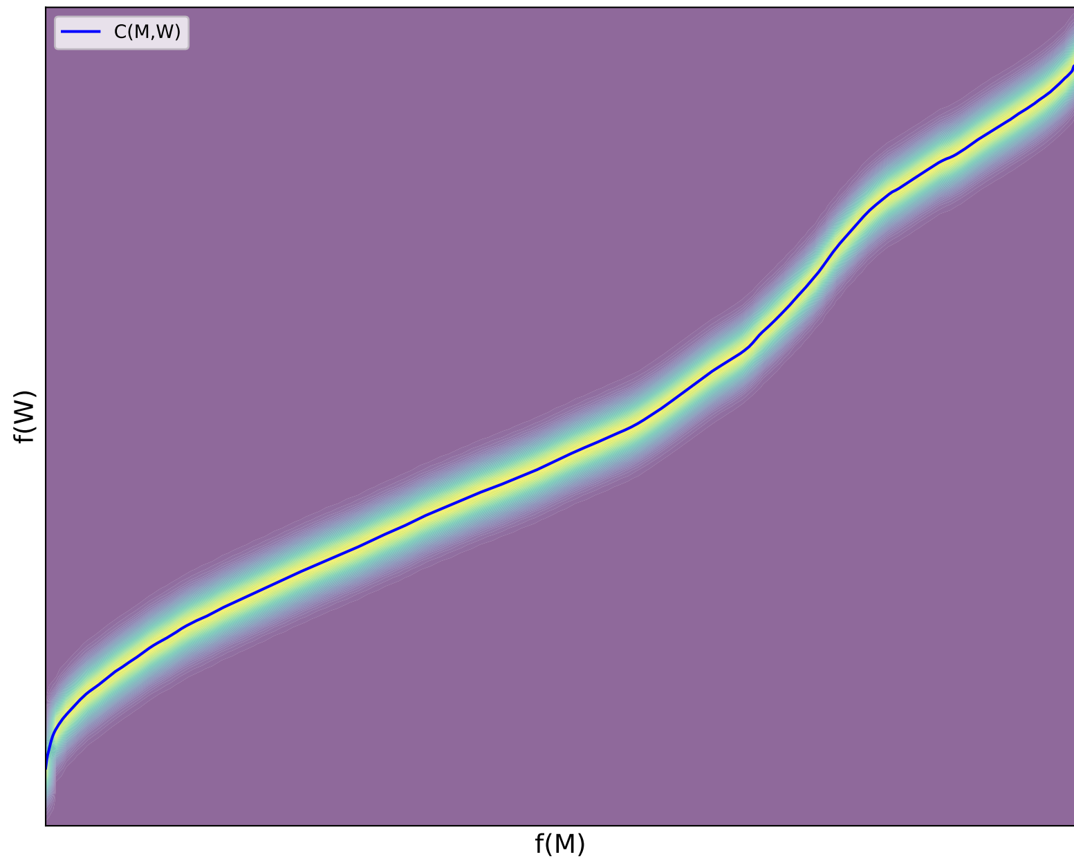
2D Normal Prior based on (M,W)
