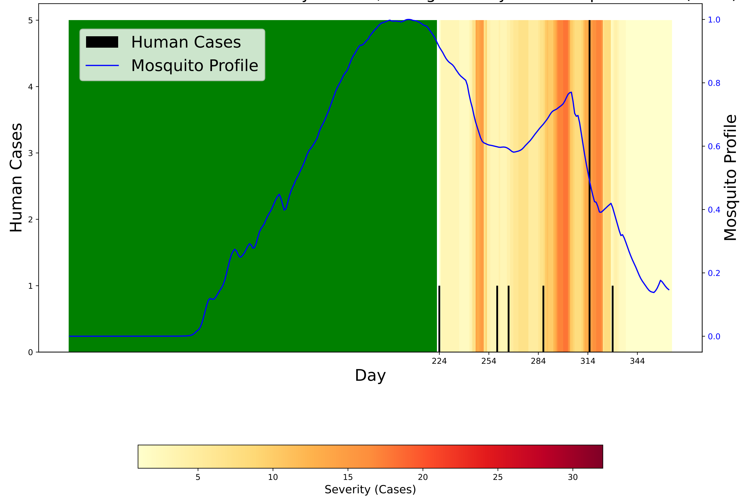
Short-term Risk Prediction for Severity of WND, Orange County with Mosquito Profile (2022)
