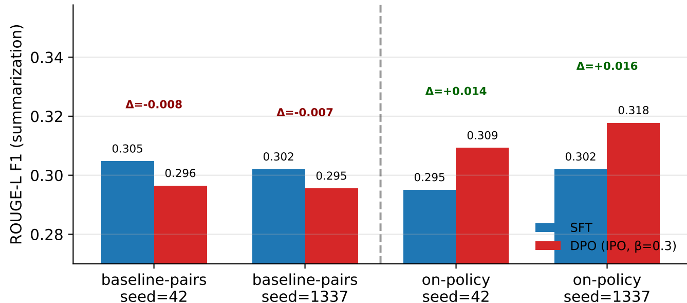
Multi-seed apples-to-apples ablation: baseline-pairs vs on-policy (seed=42 и seed=1337)
