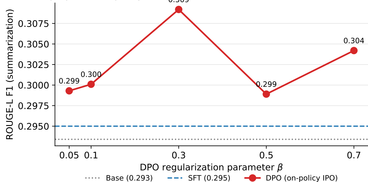
\beta -кривая on-policy DPO на summarization (seed=42, n=5 точек)
