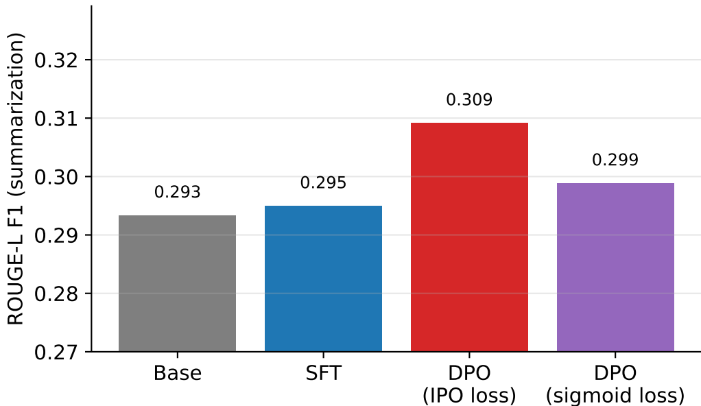
Sigmoid vs IPO при on-policy preference-pairs ( \beta=0.3 , seed=42)
