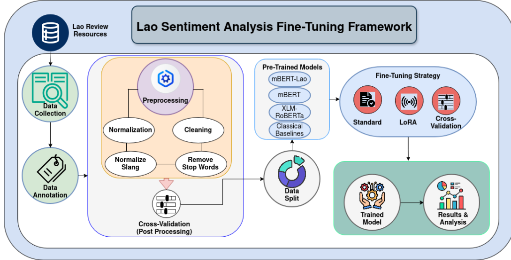
Fig. 2. Overall methodology framework for Lao sentiment classification, including dataset preparation, model selection, and fine-tuning strategies.
