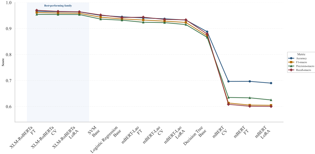
Fig. 3. Metric comparison across PLM settings and classical baselines, sorted by F1-macro.
