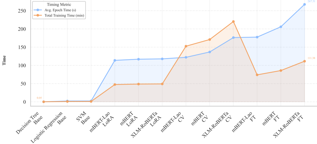
Fig. 6. Timing comparison across PLM settings and classical baselines, sorted by average epoch time.
