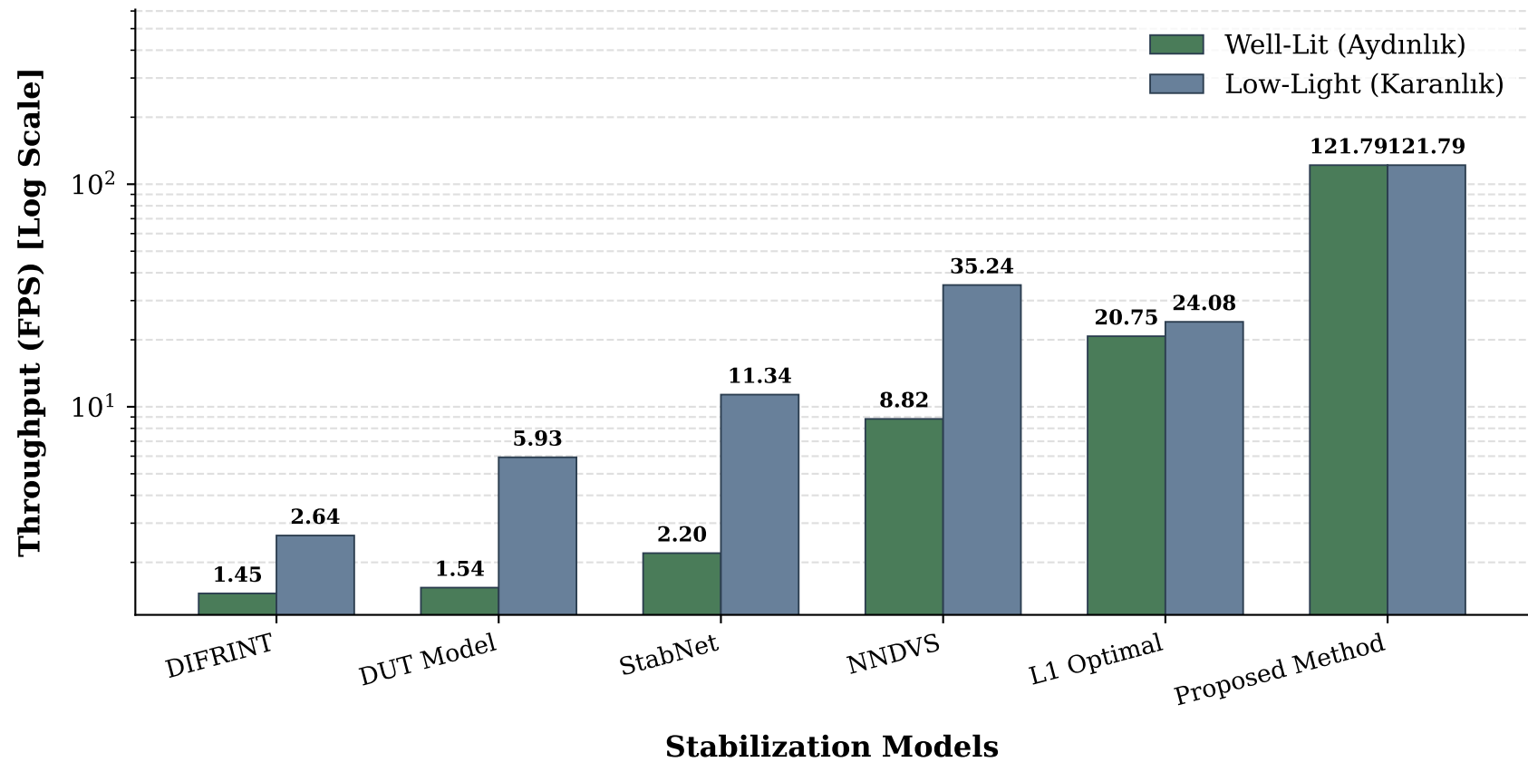
Throughput Comparison Under Varying Illumination Conditions
