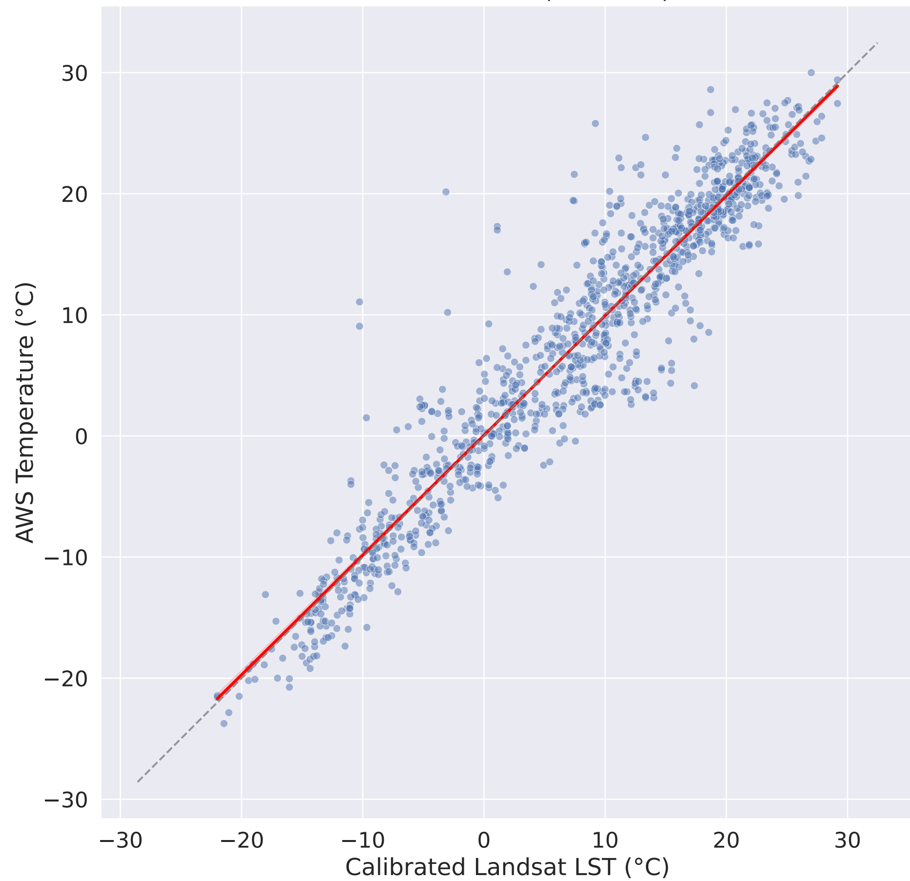
After Calibration (Test Data)
