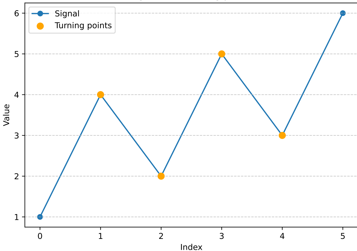
Signal with turning points
