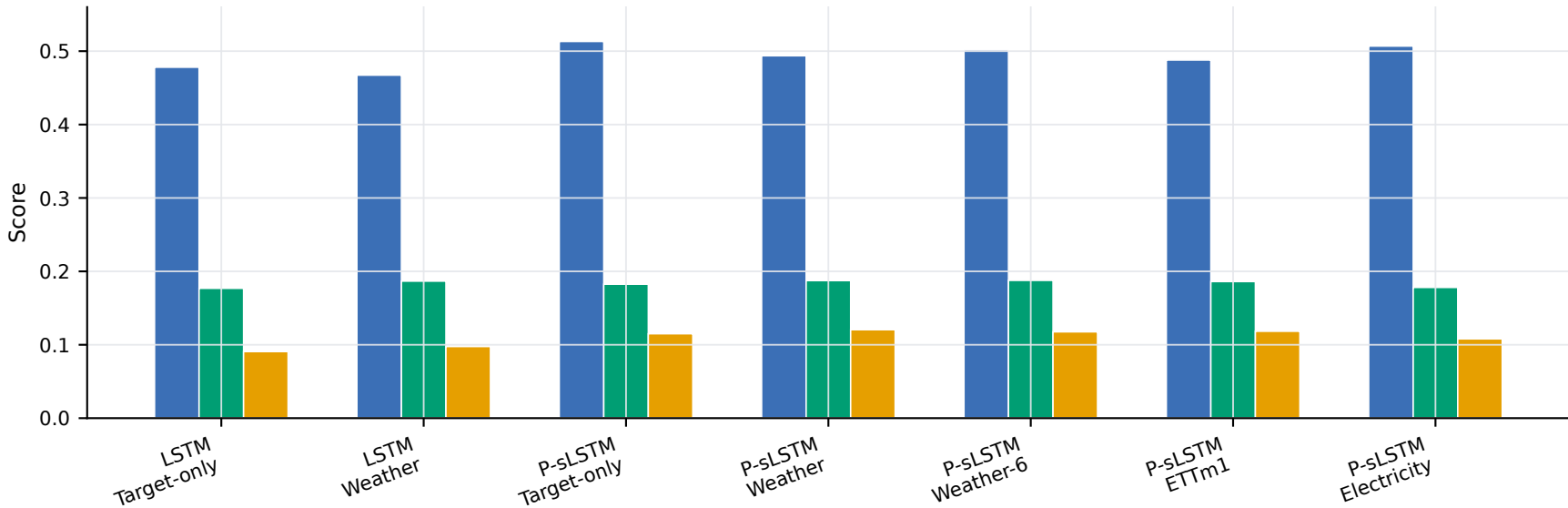
Directional Accuracy 6-Class Accuracy Macro F1 Out-of-time 2019 metrics
