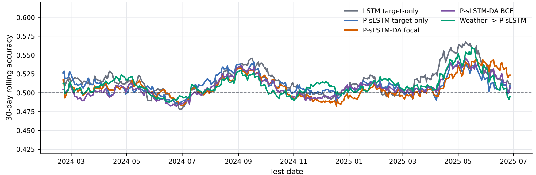
Rolling cross-sectional direction accuracy
