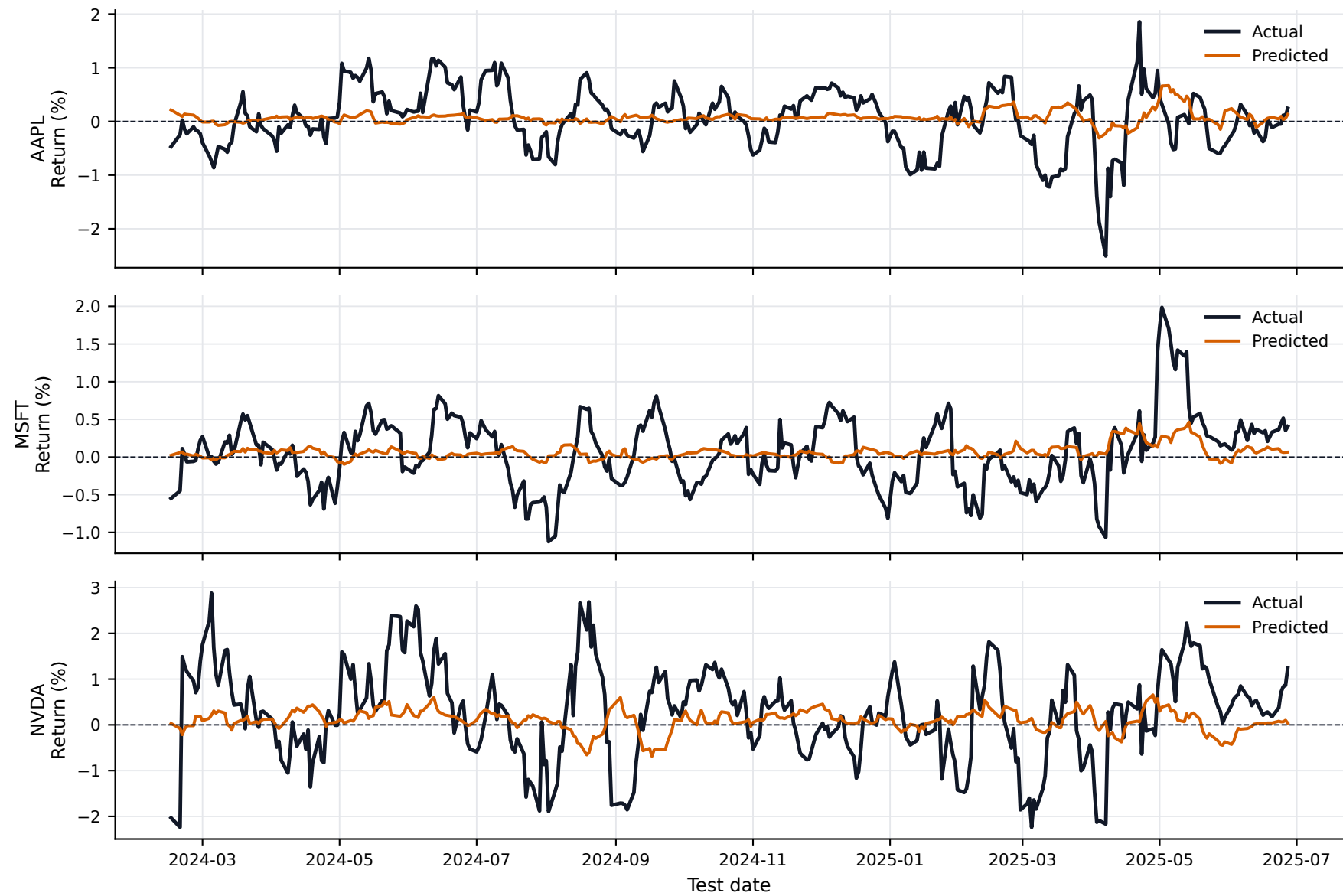
Single-stock actual vs predicted return curves (P-sLSTM-DA focal)
