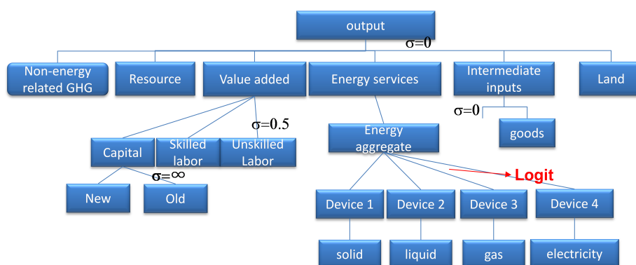
Figure 3.3: Production structure (Non-energy transformation sectors) with enduse option
