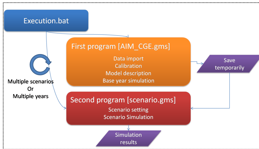
Figure 6.1: Overview of the program structure
