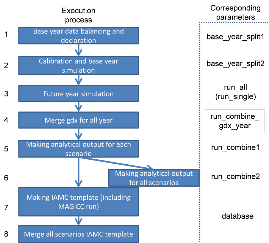
Figure 6.3: Process flow of the AIM/CGE model execution and corresponding parameters
