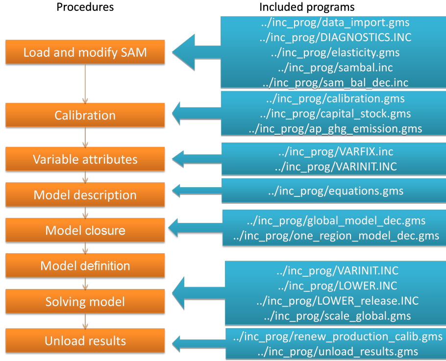
Figure 6.2: AIMHub.gms structure
