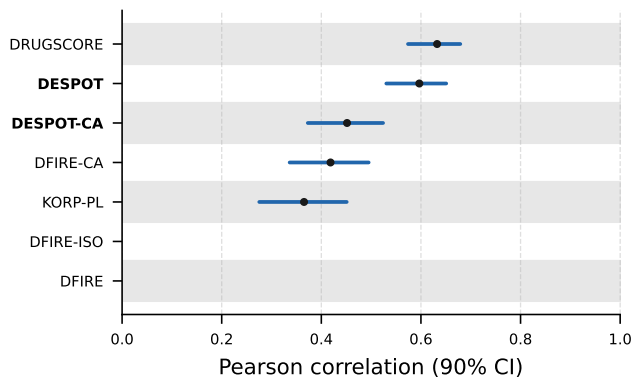
(A) Scoring power
