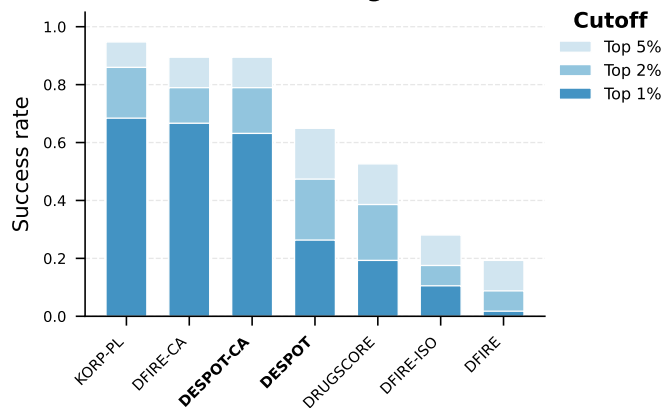
(E) Forward screening
