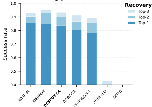
(C) Docking power
