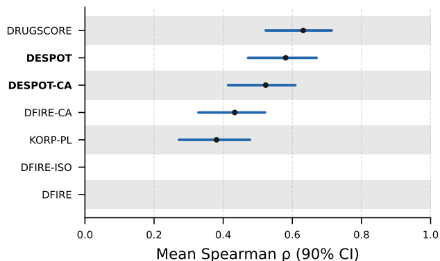
(B) Ranking power
