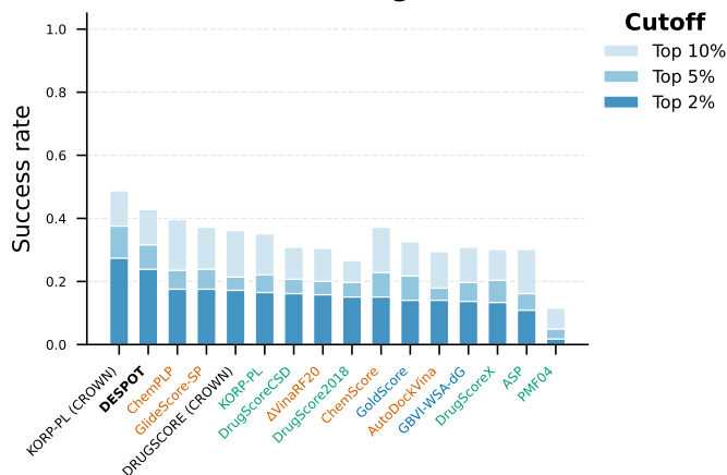
(F) Reverse screening
