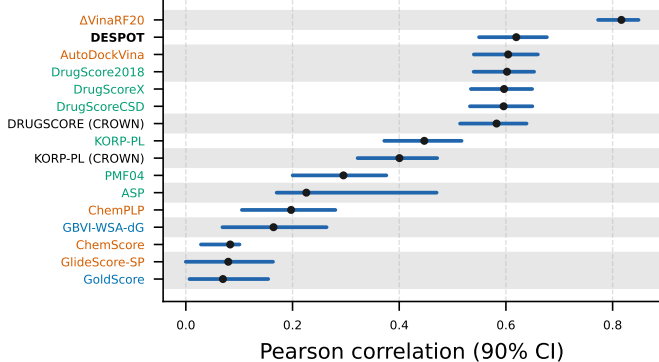
(A) Scoring power
