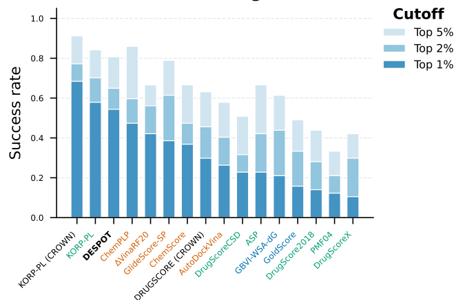
(E) Forward screening
