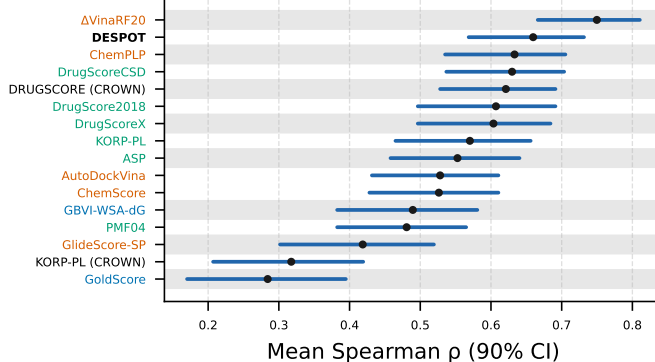
(B) Ranking power
