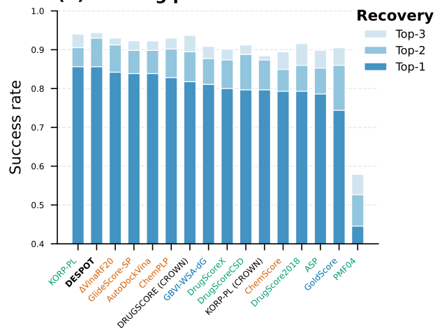
(C) Docking power
