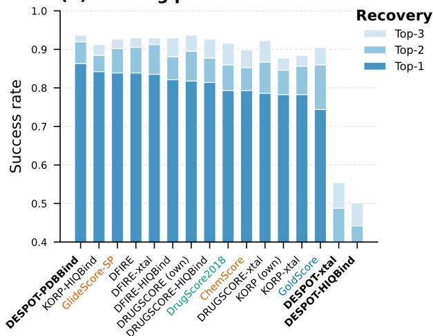
(C) Docking power
