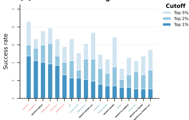
(E) Forward screening
