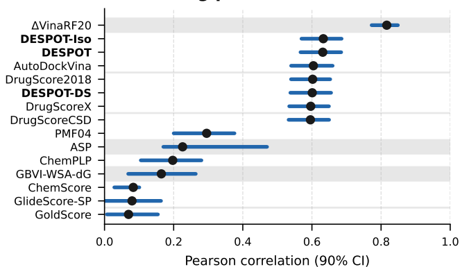
(A) Scoring power
