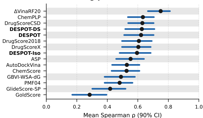
(B) Ranking power
