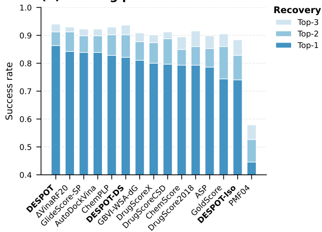
(C) Docking power
