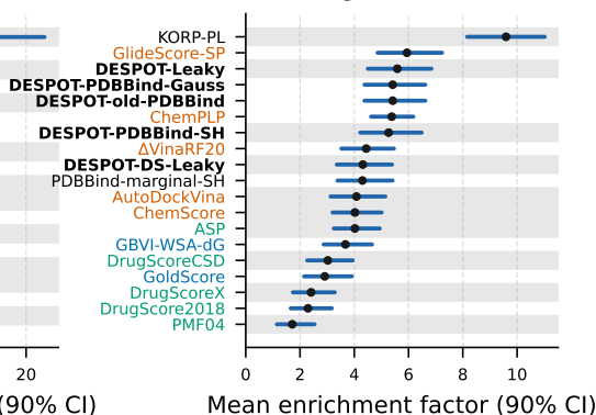
(I) EF @ 5%
