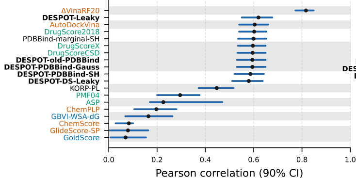
(A) Scoring power
