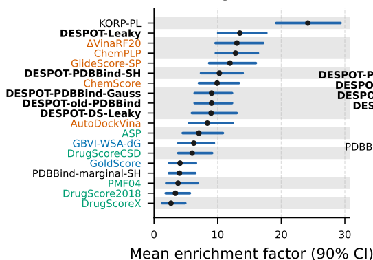
(G) EF @ 1%
