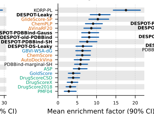
(H) EF @ 2%
