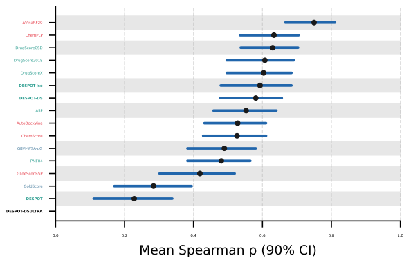
(B) Ranking power
