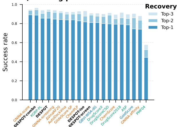
c) Docking power
