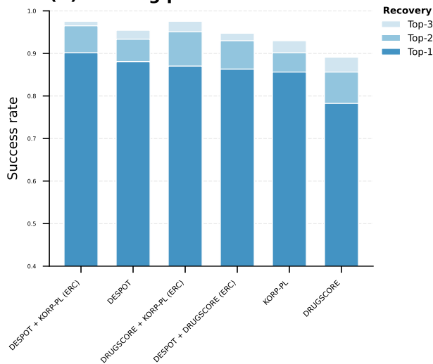
(A) Docking power
