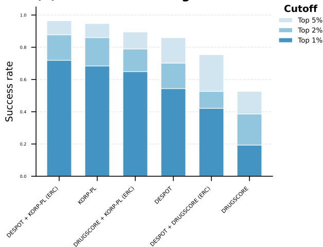
(C) Forward screening
