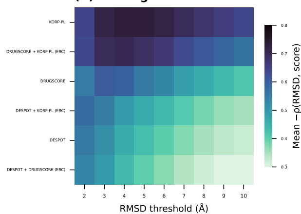
(B) Binding funnel
