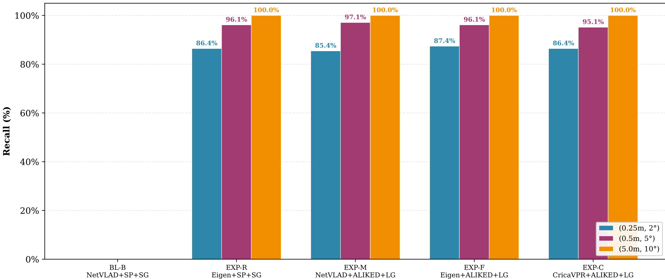
ShopFacade (Cambridge) — Recall Comparison Across Experiments
