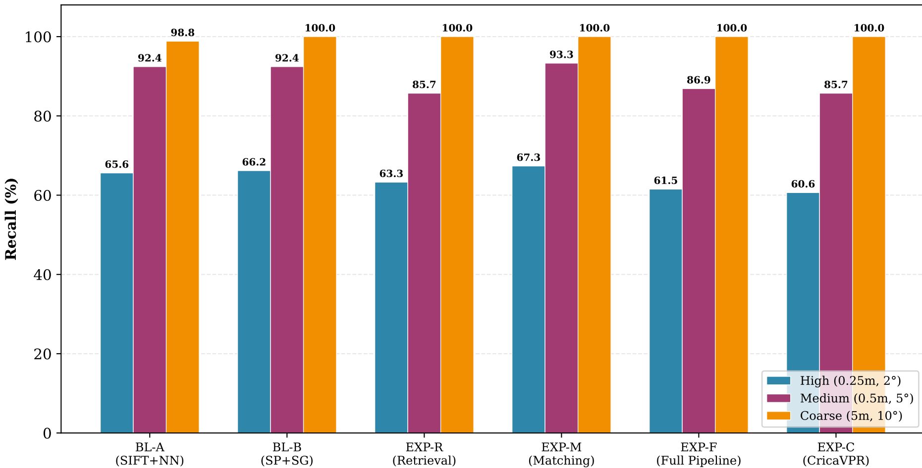
Ablation Study — Per-Module Impact on Recall
