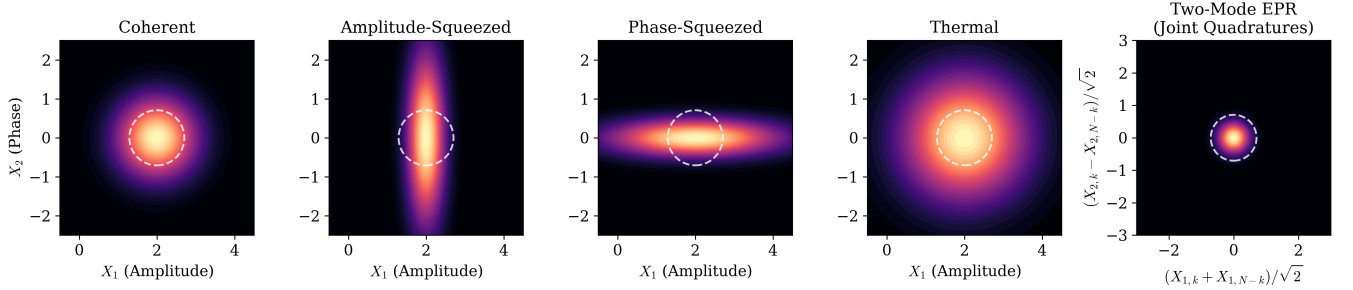
FIG. 2. Wigner phase-space distributions for the five Gaussian input states. The dashed white circle is the vacuum shot-noise reference ( \text{Var} = 1/2 ). The single-mode geometries (coherent, amplitude-squeezed, phase-squeezed, and thermal) are plotted in the local (X_1, X_2) quadrature basis at coherent displacement \alpha_k = 2.0 . The two-mode EPR state is plotted in the joint sum/difference quadrature basis, where the squeezing manifests in the correlated macroscopic observables.
