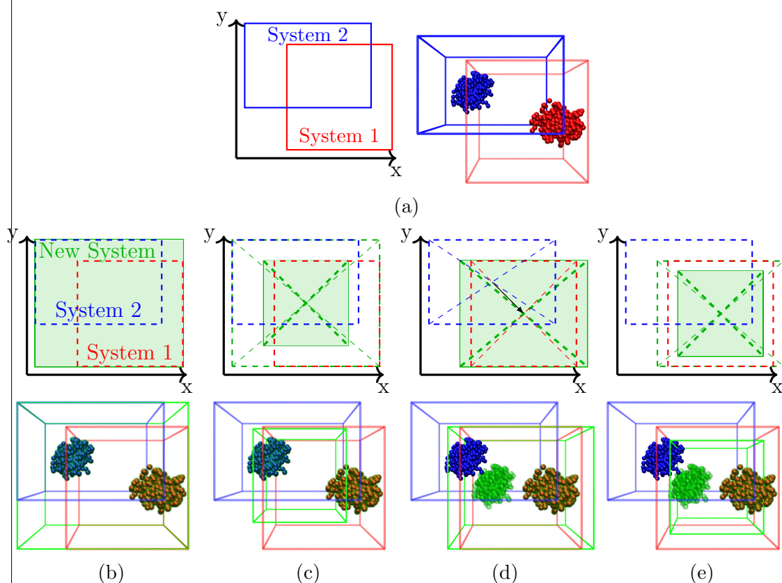
Figure 3.3: Schematic representation and corresponding snapshots illustrating JoinSystems behaviour. (a) The original systems: System1.lampstrj (red) and System2.lampstrj (blue) in the Examples/JoinSystems folder. The rest show examples of possible options (green rectangles and transparent balls represent the new systems): (b) no options; (c) -b 20 20 20 option; (d) -off c c c ; (e) -b 20 20 20 -off c c c , i.e., combining (c) and (d). These new systems are in the Examples/JoinSystems folder as NewSystem\_#\#.lampstrj , where \# is b, c, d, or e.
