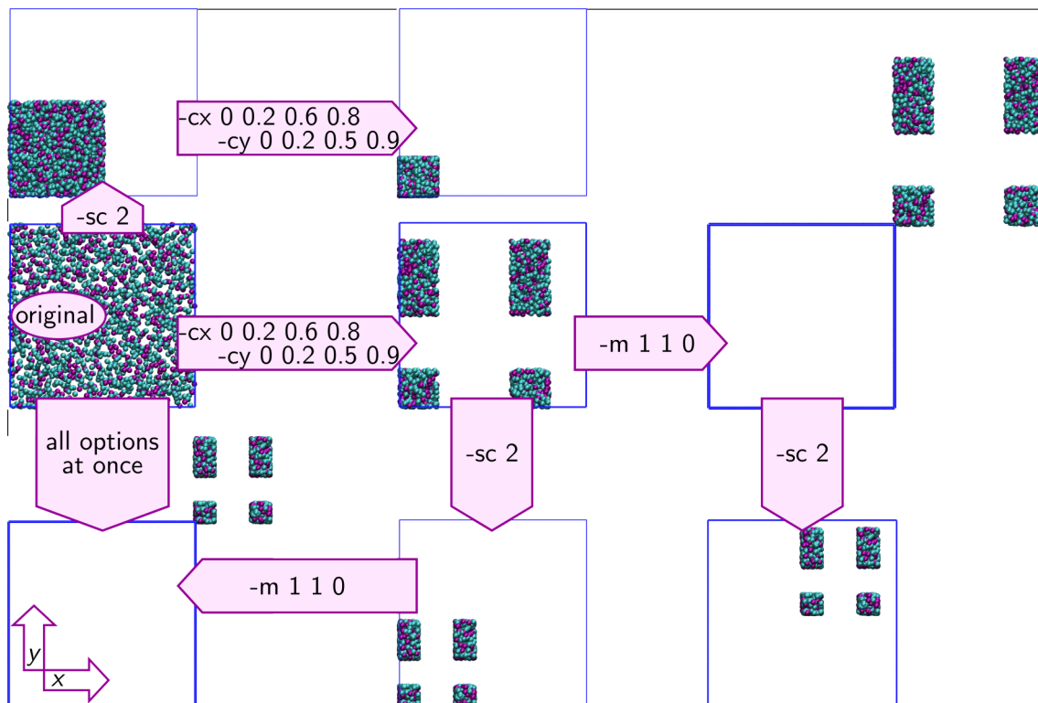
Obrázek 3.4: Some of the possible results when combining sequential runs of the Selected utility, namely (1) constraining x and y coordinates via -cx 0 0.2 0.6 0.8 -cy 0 0.2 0.5 0.9 , (2) scaling (dividing) coordinates via -sc 2 , and (3) moving coordinates via -m 1 1 0 . The blue lines represent the simulation box (the varying line thickness is just an artefact of how the snapshots were created in vmd ).
