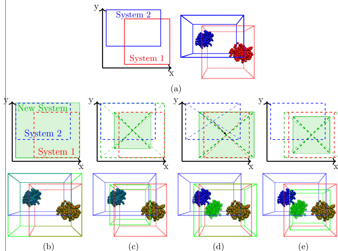
Obrázek 3.3: Schematic representation and corresponding snapshots illustrating JoinSystems behaviour. (a) The original systems: System1.lampstrj (red) and System2.lampstrj (blue) in the Examples/JoinSystems folder. The rest show examples of possible options (green rectangles and transparent balls represent the new systems): (b) no options; (c) -b 20 20 20 option; (d) -off c c c ; (e) -b 20 20 20 -off c c c , i.e., combining (c) and (d). These new systems are in the Examples/JoinSystems folder as NewSystem\_#\_#.lampstrj , where \# is b, c, d, or e.
