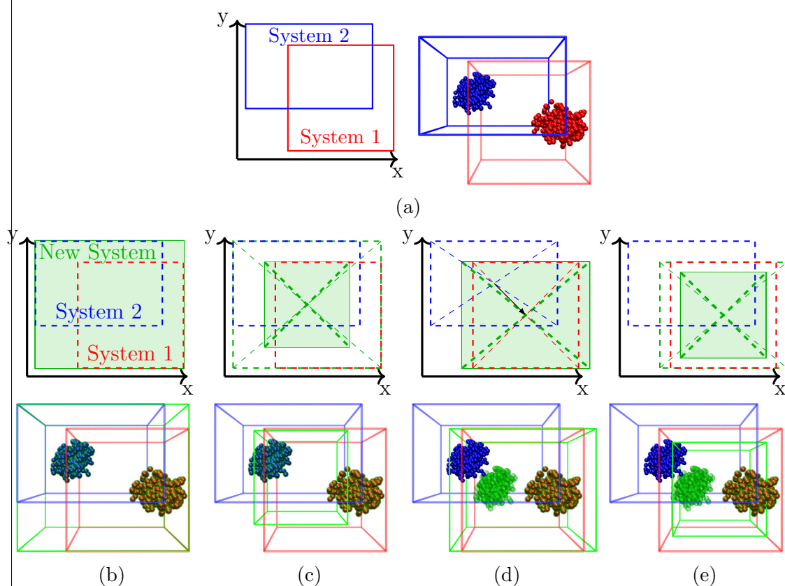
Figure 3.3: Schematic representation and corresponding snapshots illustrating JoinSystems behaviour. (a) The original systems: System1.lammppstrj (red) and System2.lammppstrj (blue) in the Examples/JoinSystems folder. The rest show examples of possible options (green rectangles and transparent balls represent the new systems): (b) no options; (c) -b 20 20 20 option; (d) -off c c c ; (e) -b 20 20 20 -off c c c , i.e., combining (c) and (d). These new systems are in the Examples/JoinSystems folder as NewSystem\_#\lammppstrj , where \# is b, c, d, or e.
