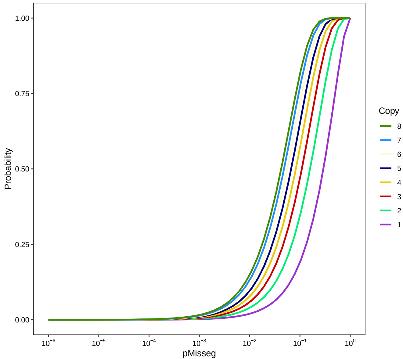
Mis-segregation probability per copy number
