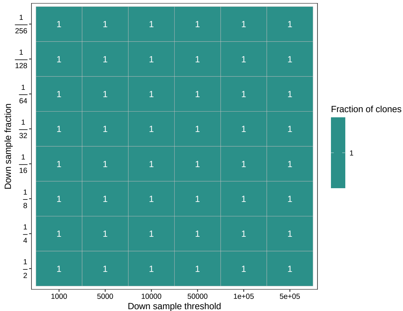
Clonal survival to 50 generation (200 clones)
