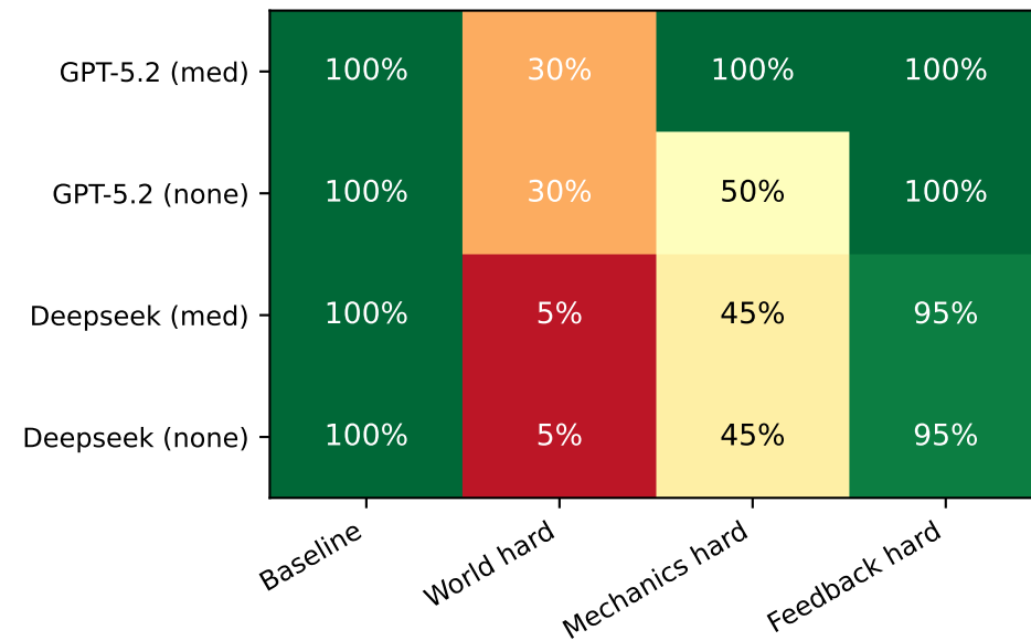
LS20
