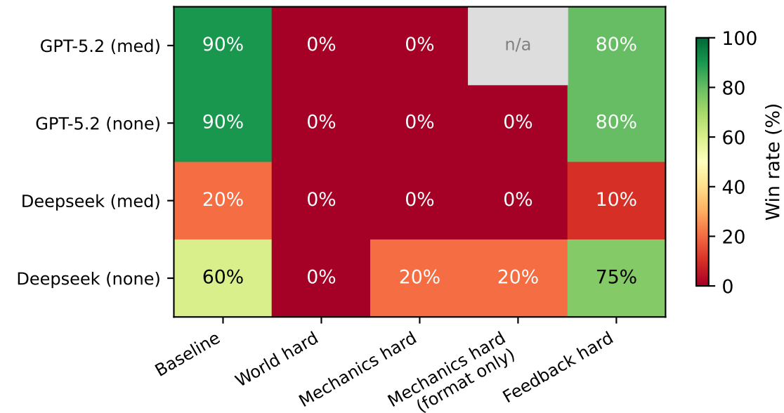
KA59-Simple
