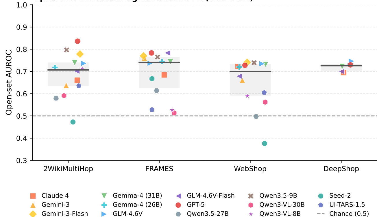
Open-set unknown-agent detection (XGBoost)
