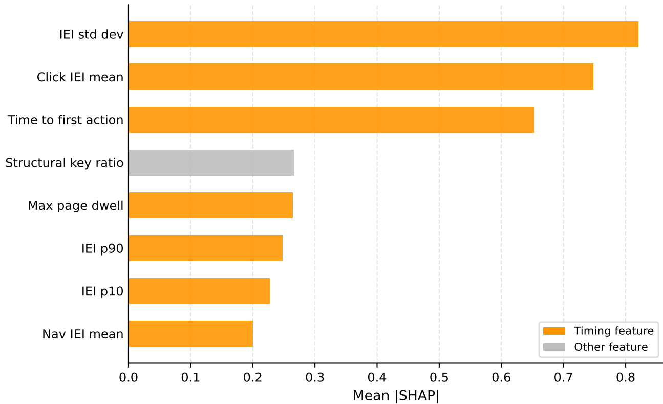
XGBoost SHAP feature importances
