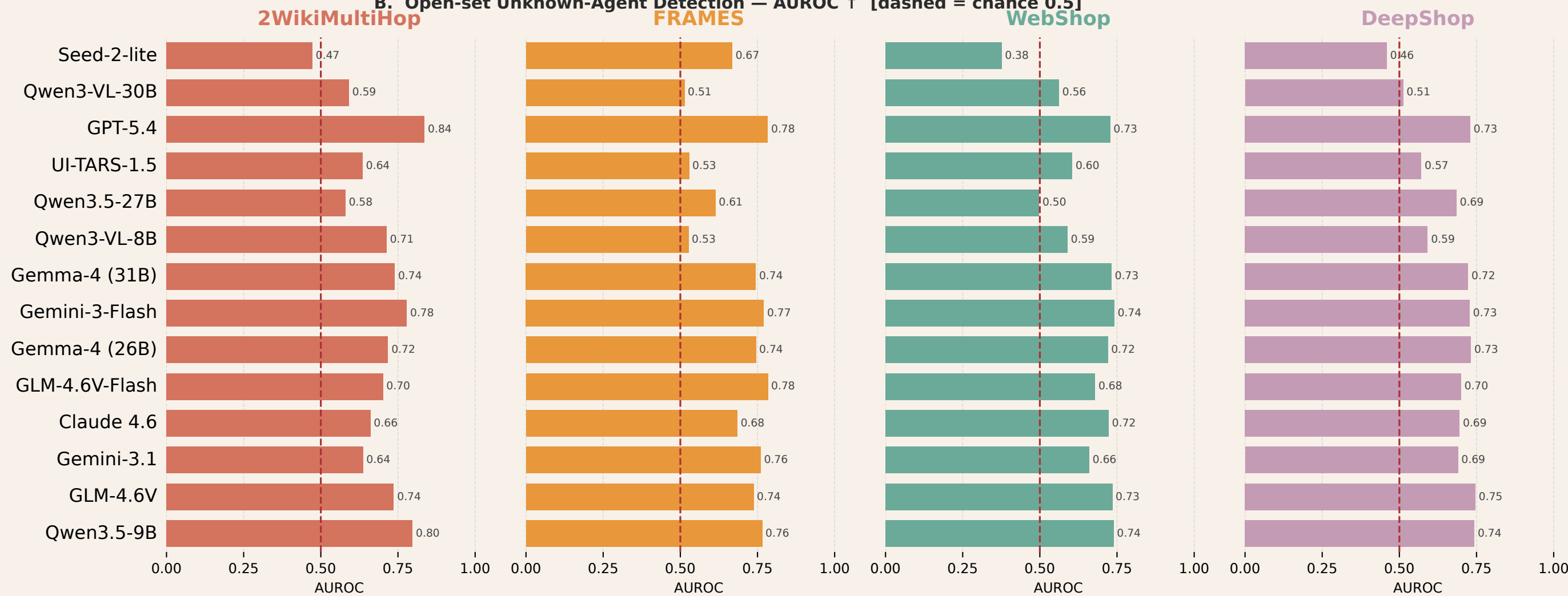
B. Open-set Unknown-Agent Detection — AUROC ↑ [dashed = chance 0.5]
