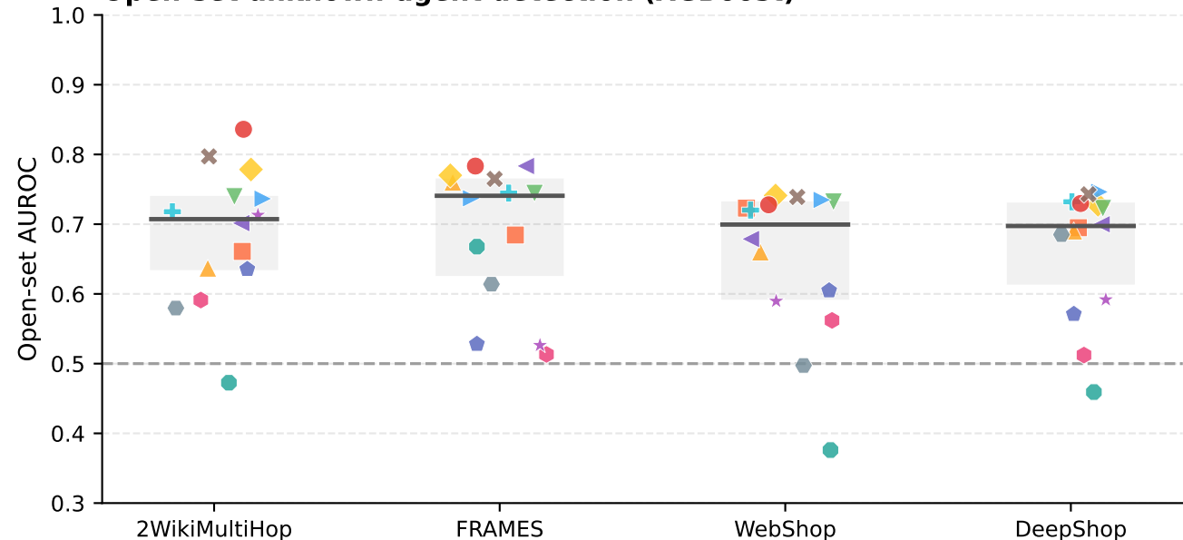
Open-set unknown-agent detection (XGBoost)
