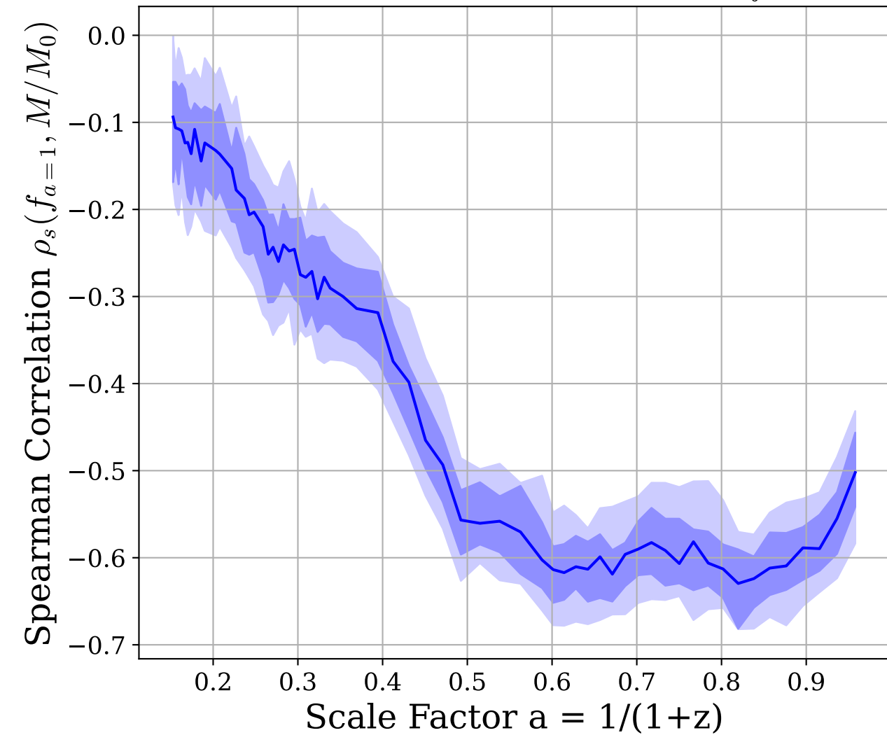
Substructure Mass Fraction f
