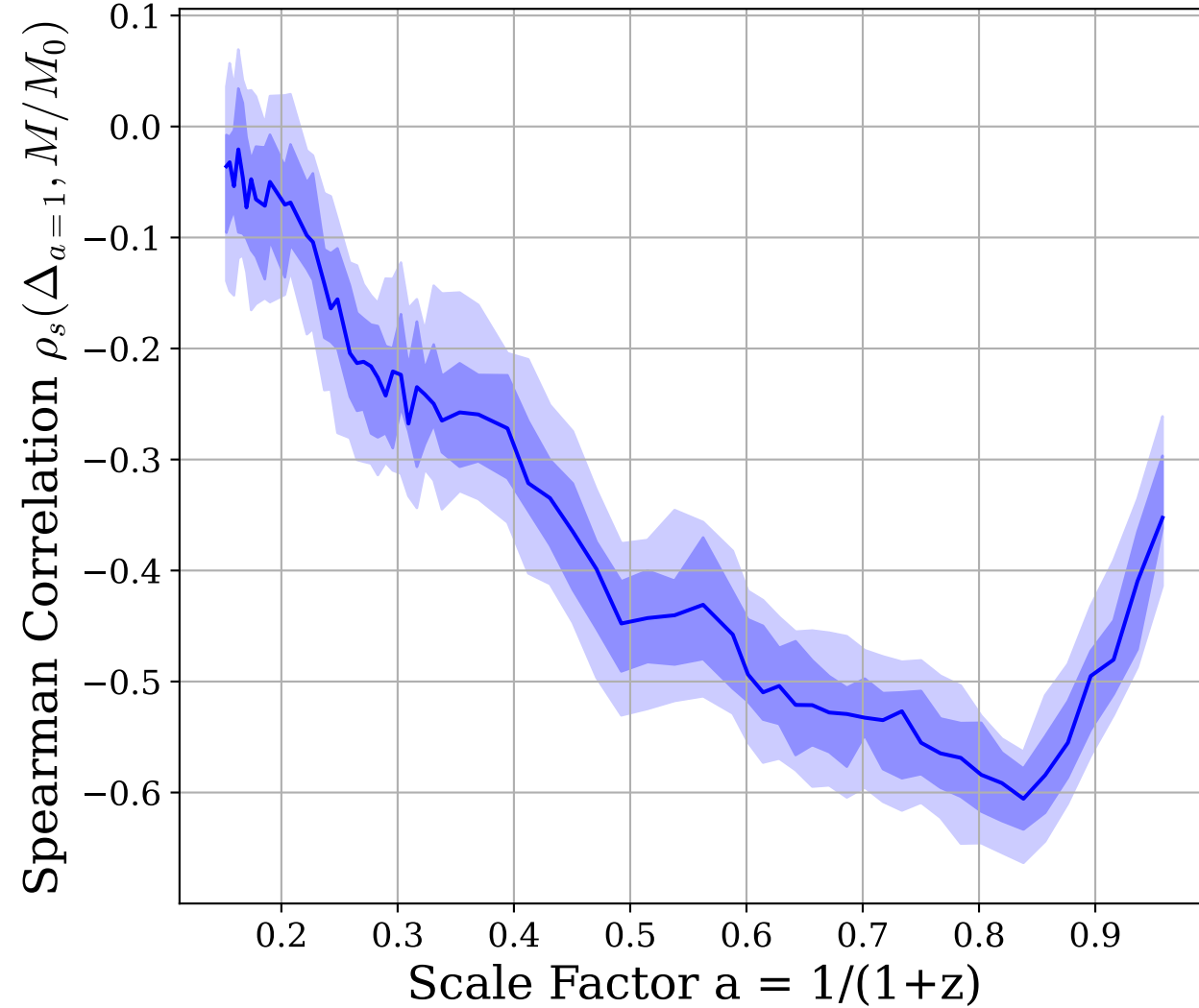
Center of Mass Offset \Delta
