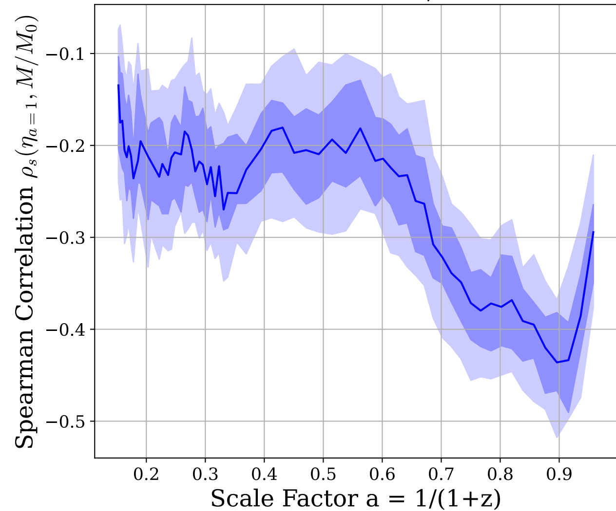
Virial Ratio \eta
