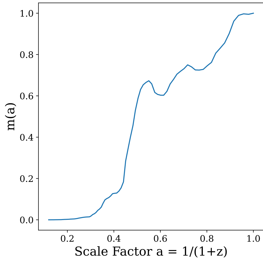
Cluster 306 | Early Formation
