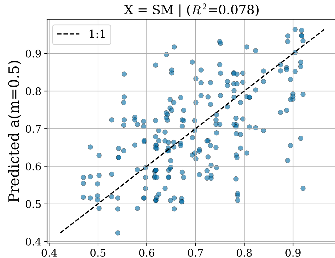
MultiCAM Predicted a(m=0.5)
