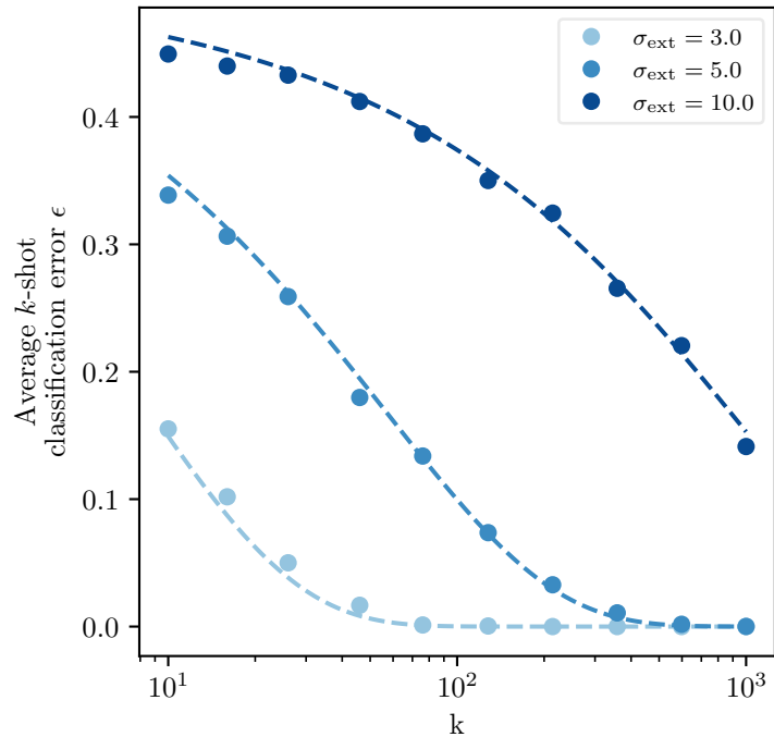
Binary Classification
