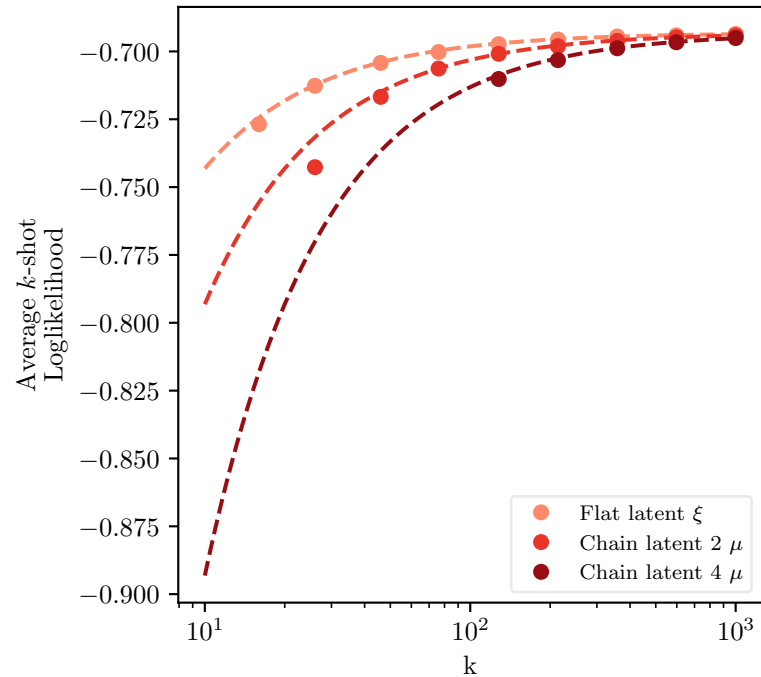
HMM
