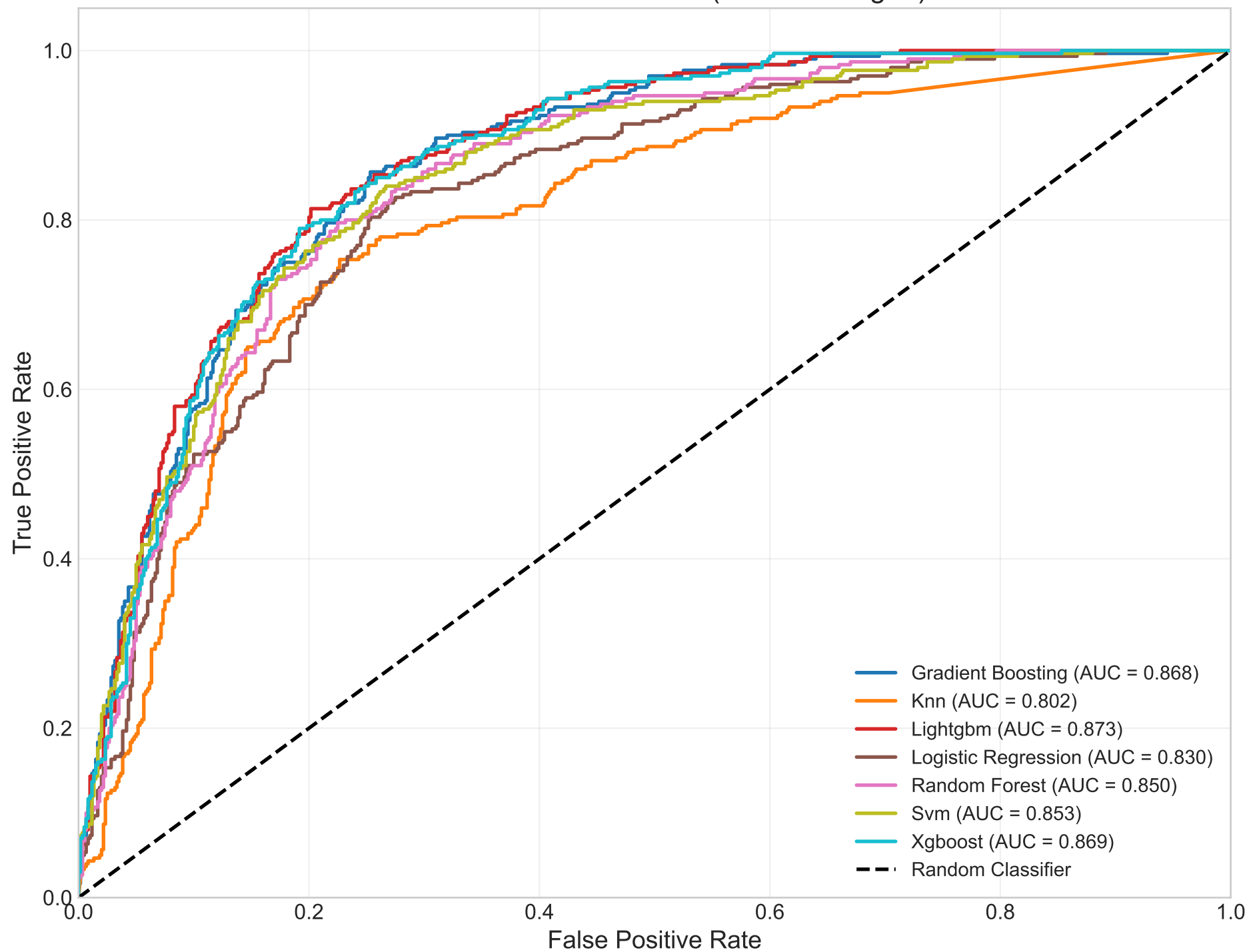
ROC Curves - Multi-class (Micro-averaged)
