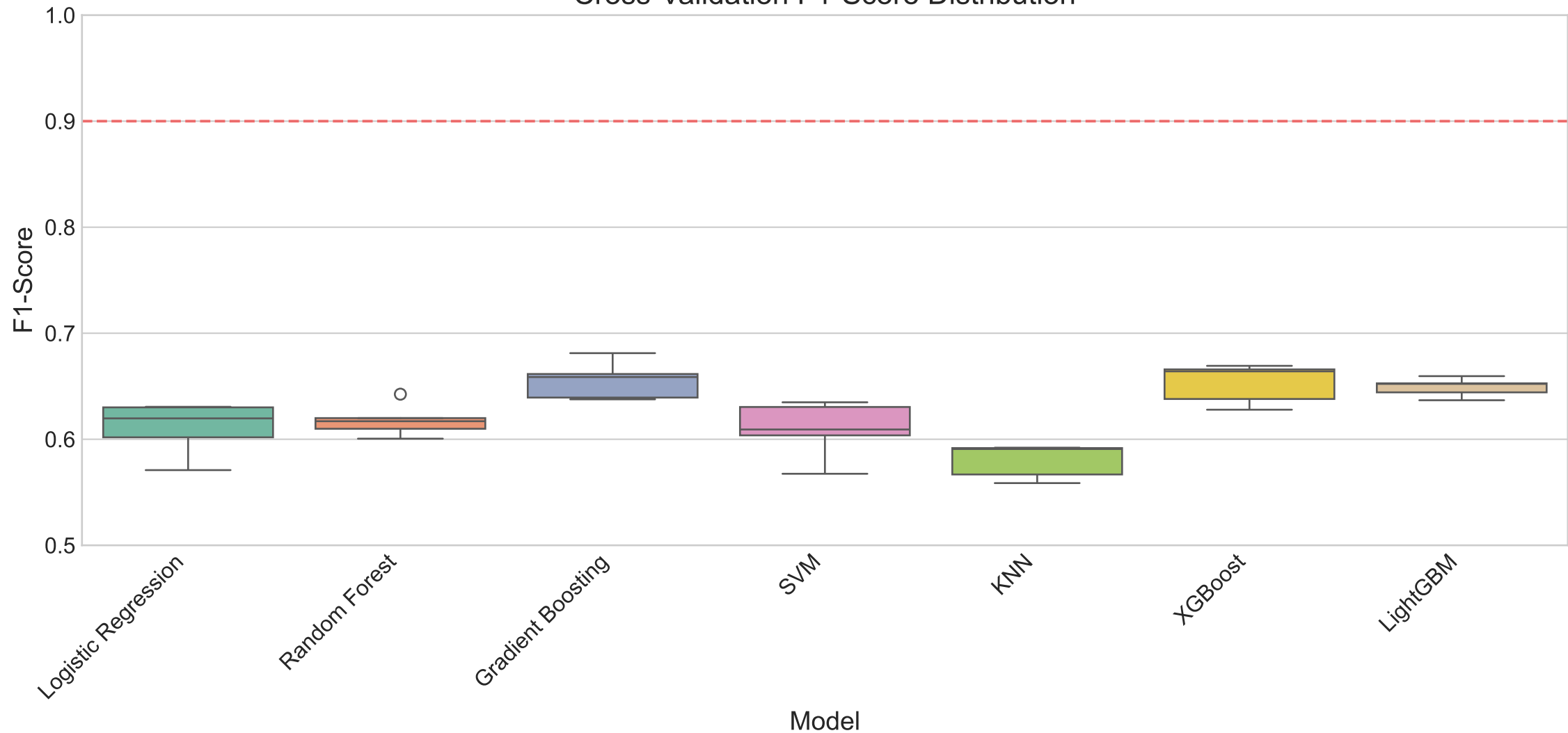
Cross-Validation F1-Score Distribution
