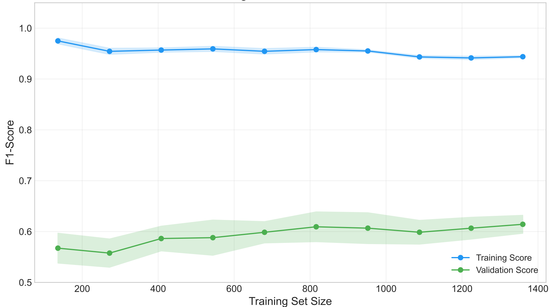
Learning Curve - Random Forest
