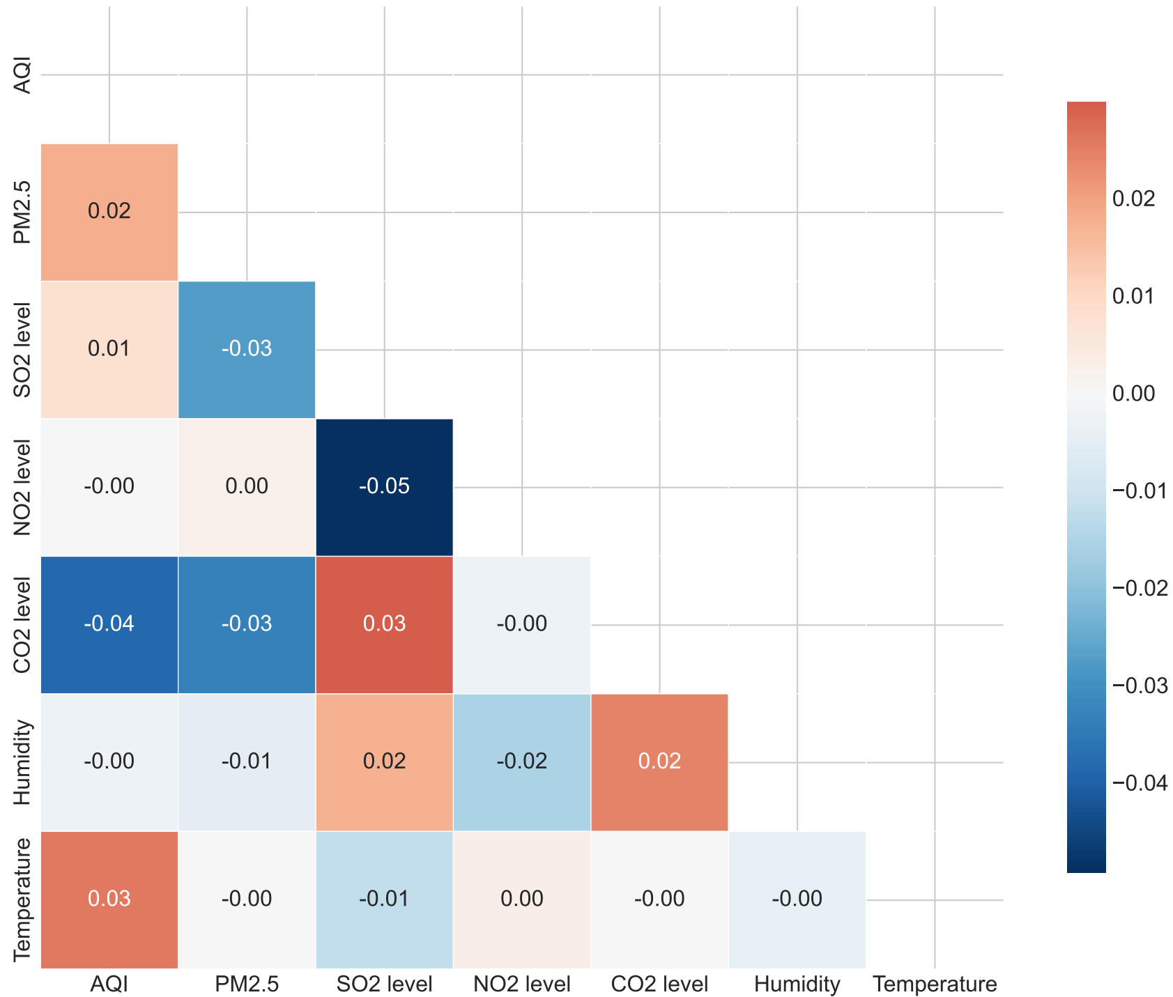
Feature Correlation Matrix
