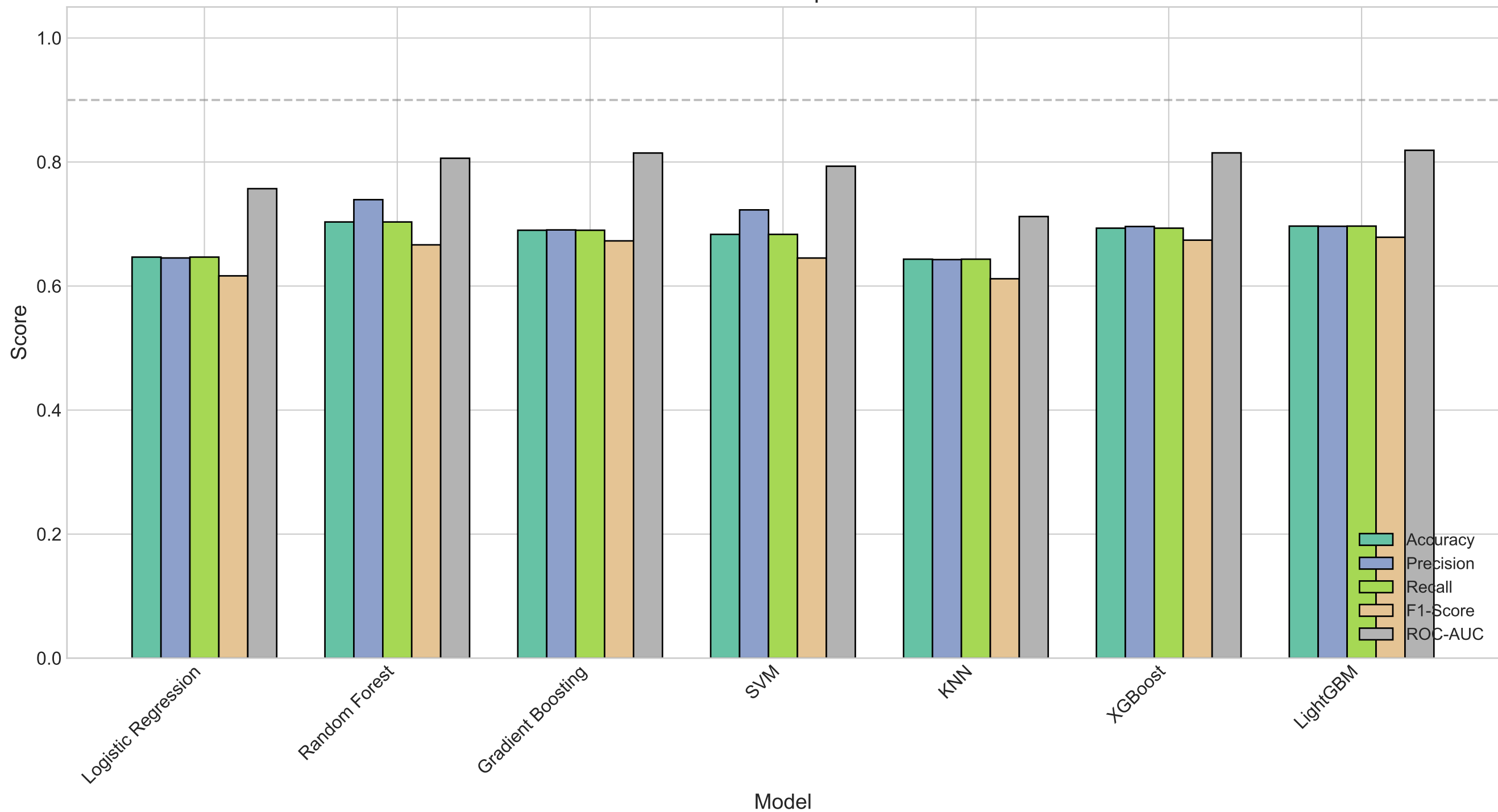
Model Performance Comparison on Test Set
