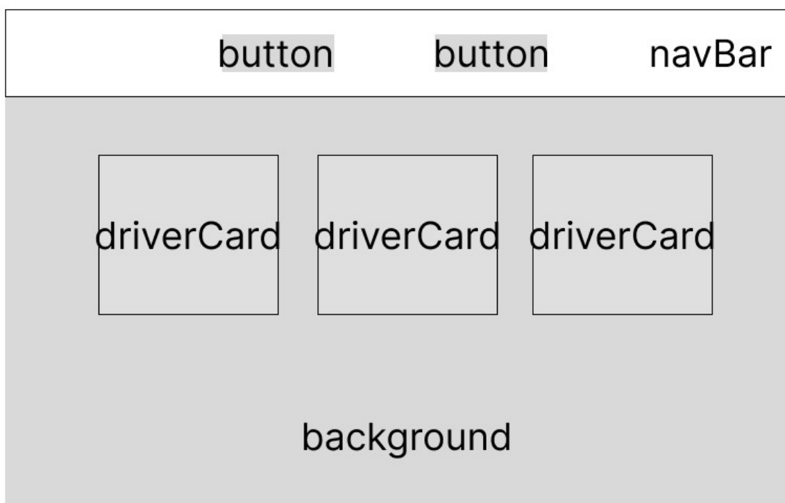
Figure 3 : Composants page pilotes
