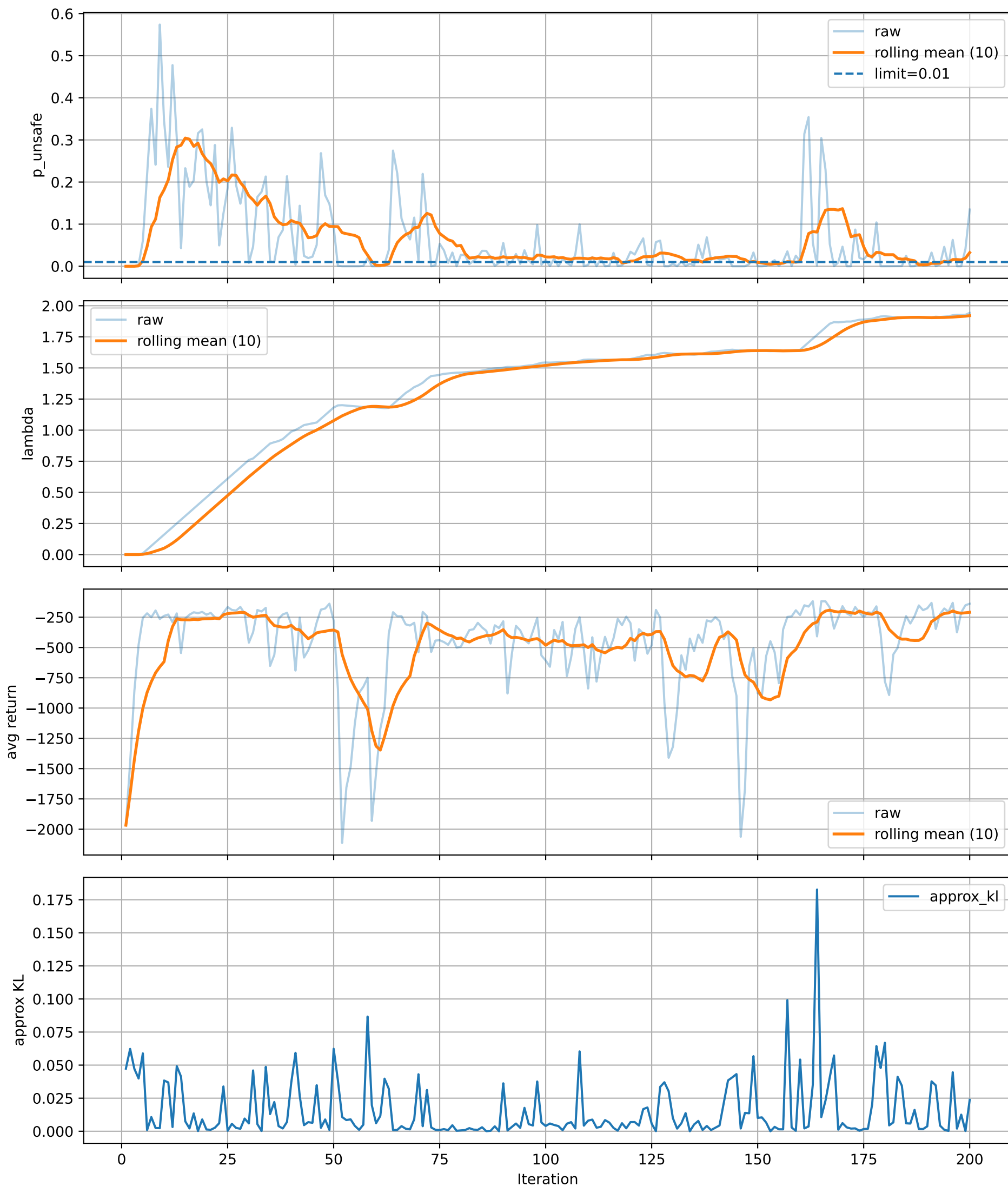
PPO-Lagrangian Training Dynamics (Safety, Dual Variable, Return, KL)
