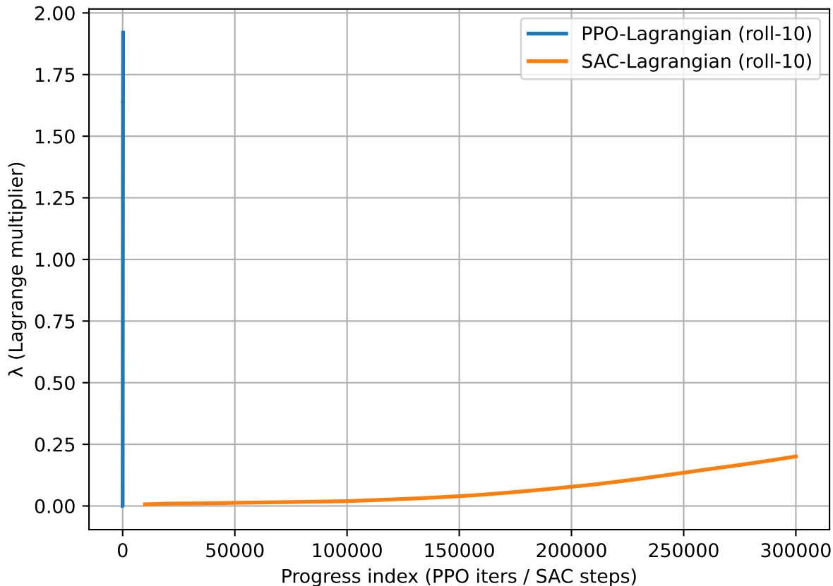
Dual Variable Evolution: PPO vs SAC
