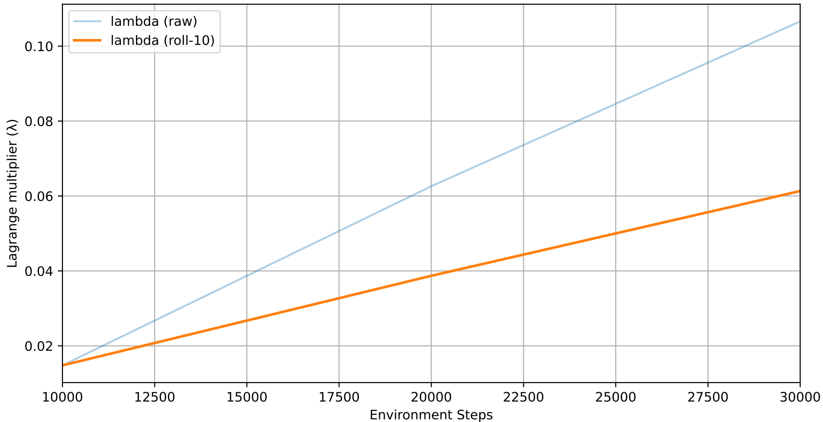
SAC-Lagrangian Dual Variable ( \lambda )
