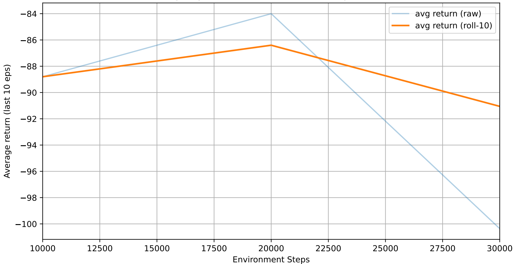
SAC-Lagrangian Performance Under Safety Constraint
