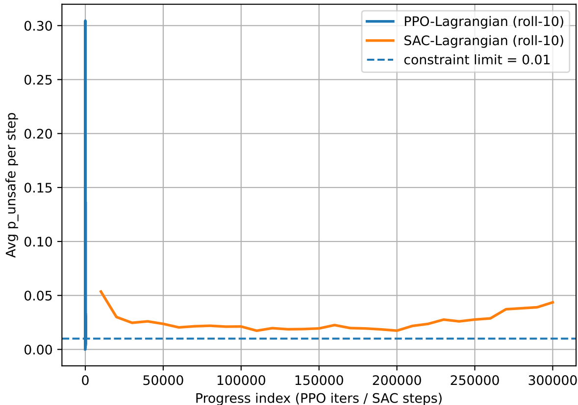
Safety Tracking: PPO vs SAC
