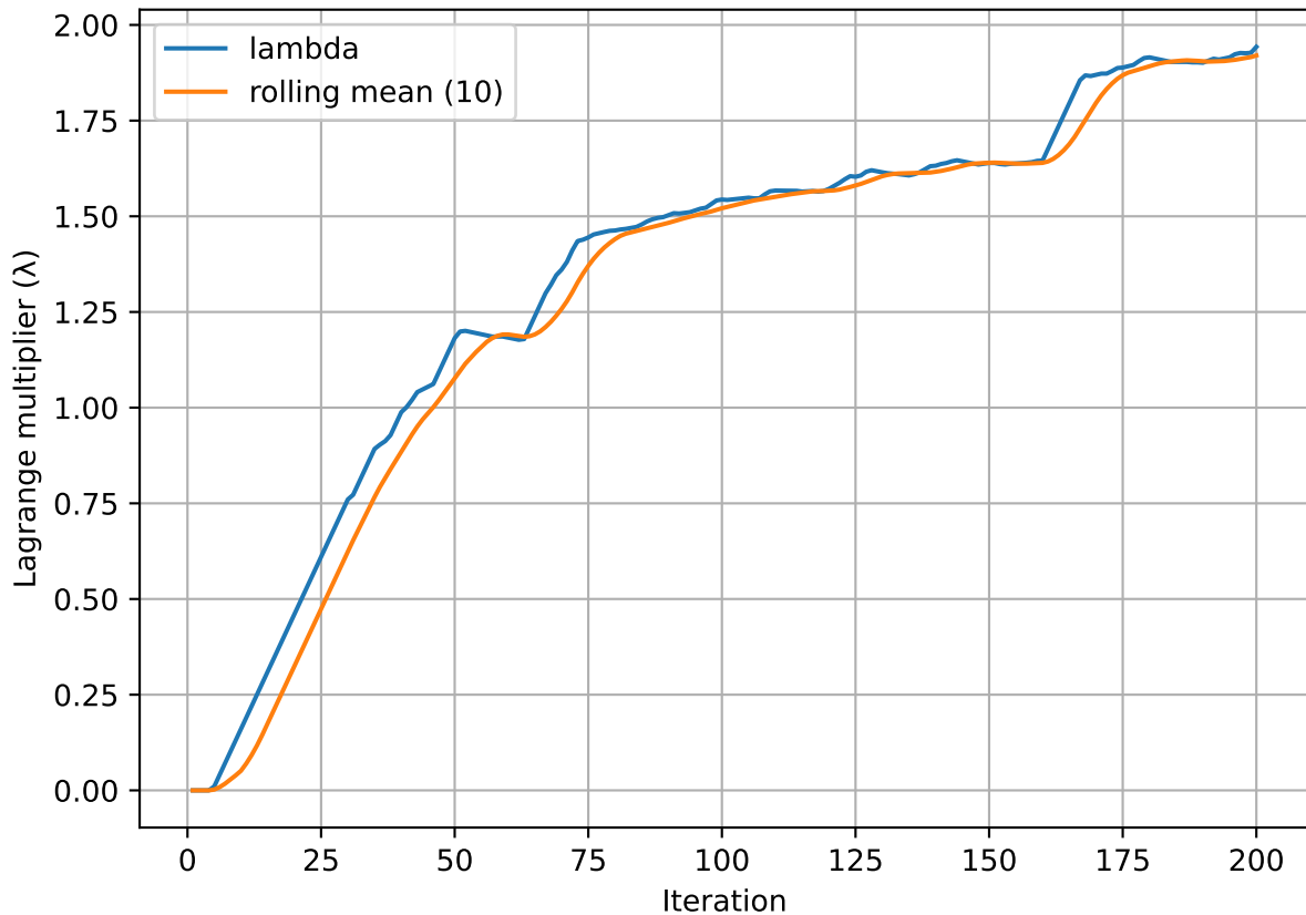
Dual Variable Evolution ( \lambda )
