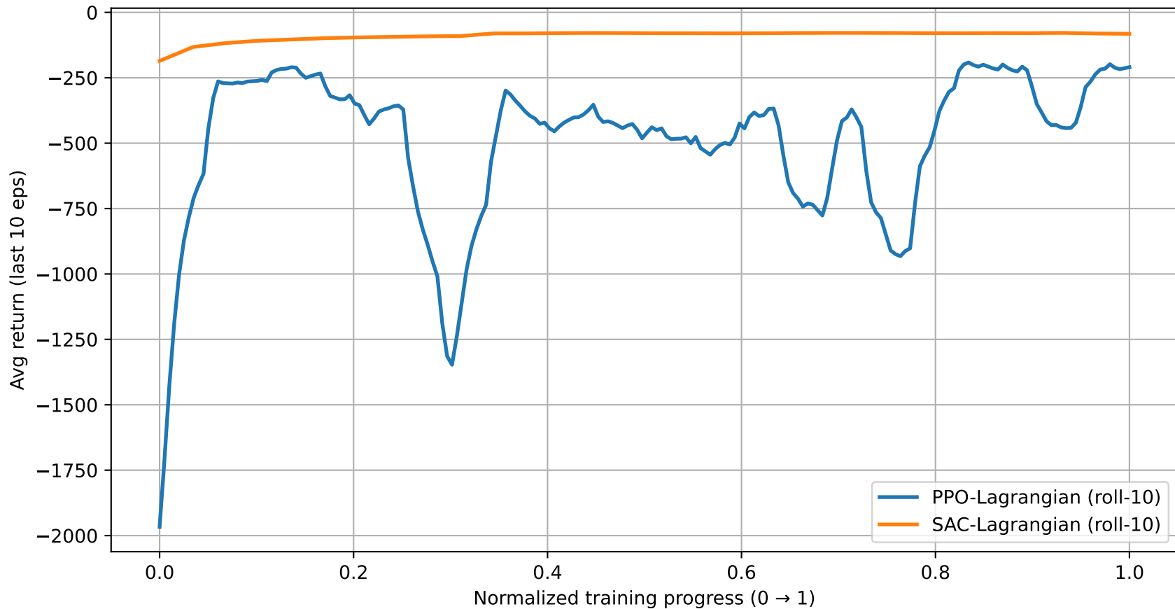
Performance (Normalized): PPO vs SAC
