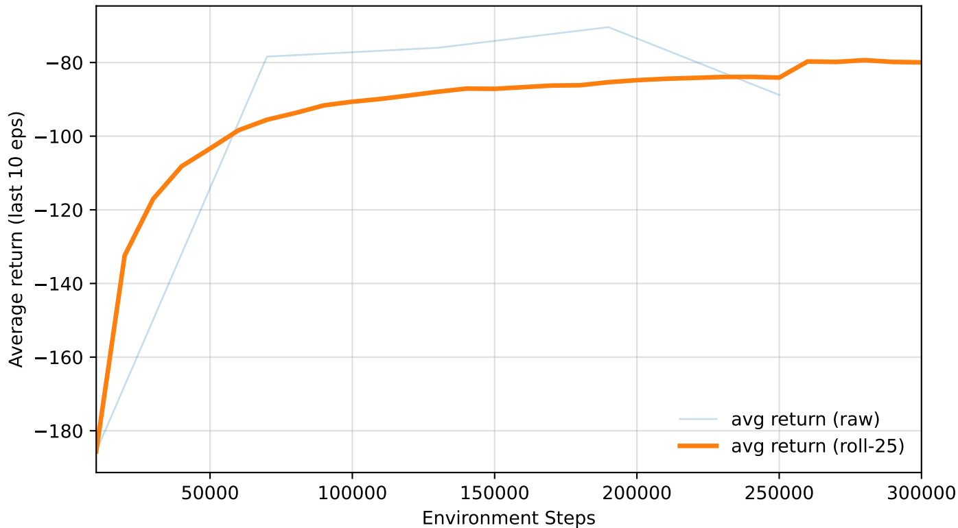
SAC-Lagrangian Performance Under Safety Constraint
