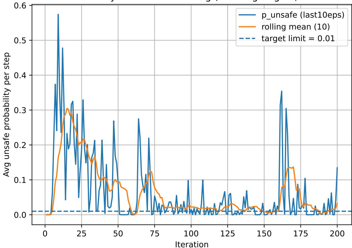
Safety Constraint Tracking (PPO-Lagrangian)
