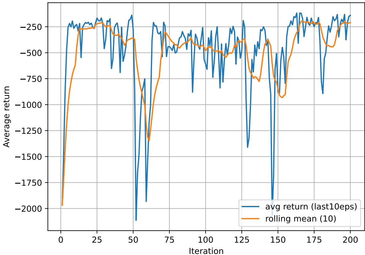
Performance Under Safety Constraint
