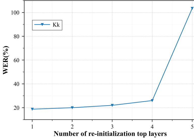
Figure 3: WER and CER values for different numbers of reinitialized top encoder layers in Karakalpik ASR.
