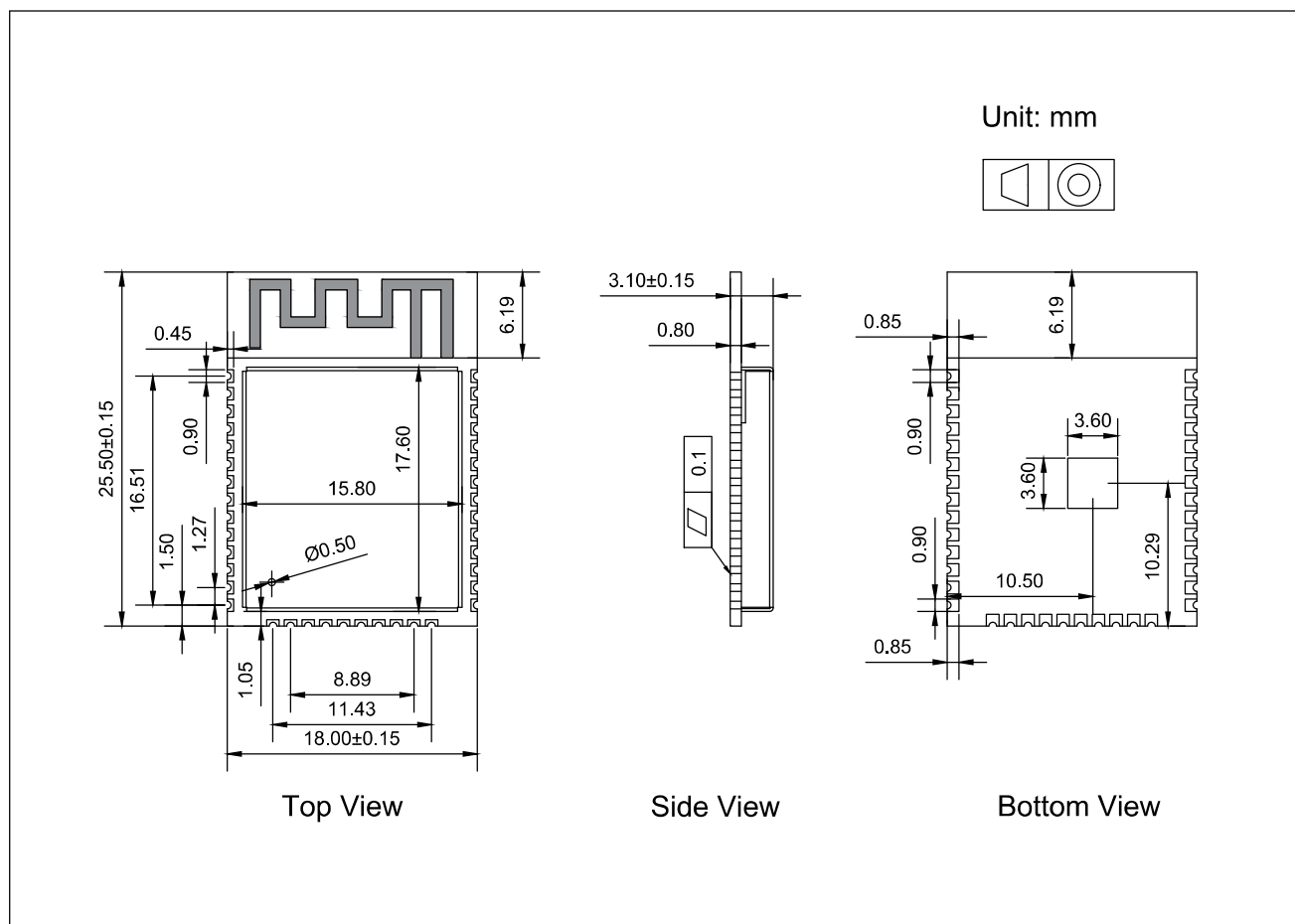
Figure 8: Physical Dimensions of ESP32-WROOM-32D
