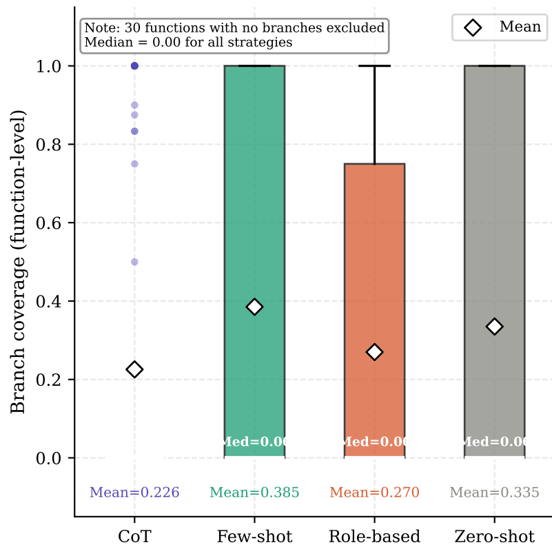
(b) Branch coverage distribution
