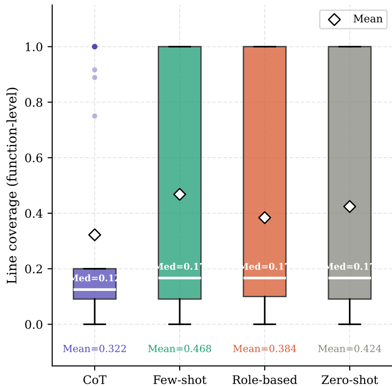
(a) Line coverage distribution
