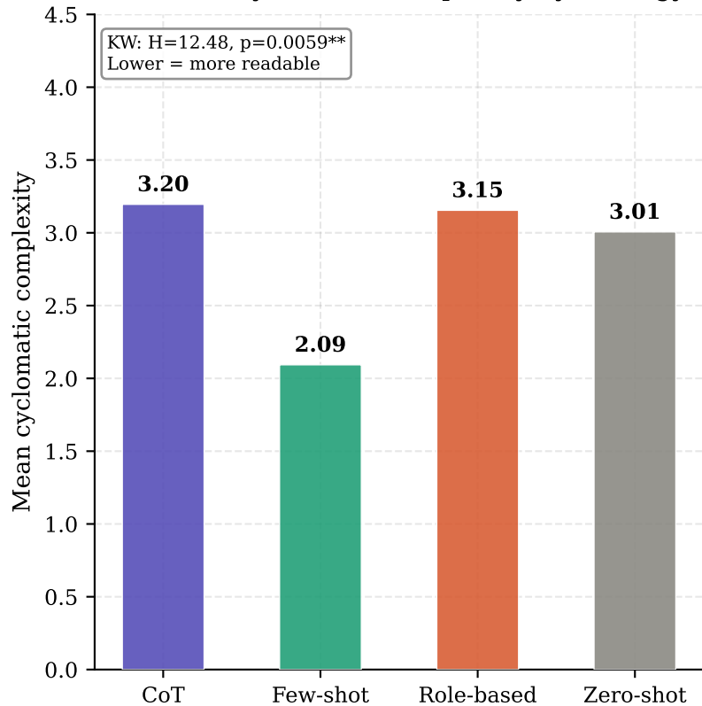
(a) Mean cyclomatic complexity by strategy
