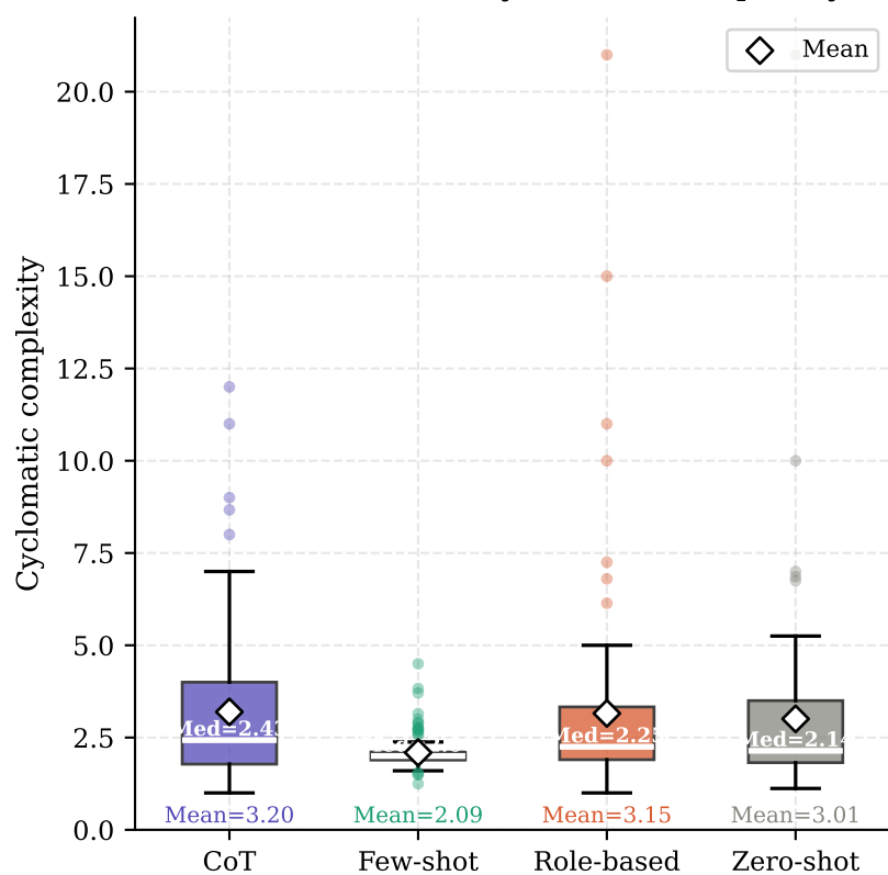
(b) Distribution of cyclomatic complexity
