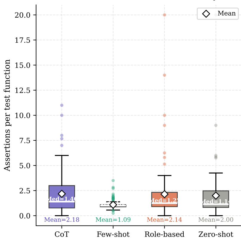
(b) Distribution of assertion density
