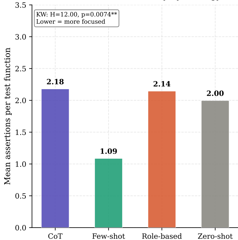
(a) Mean assertion density by strategy
