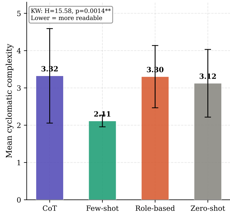
(a) Cyclomatic complexity of test functions
