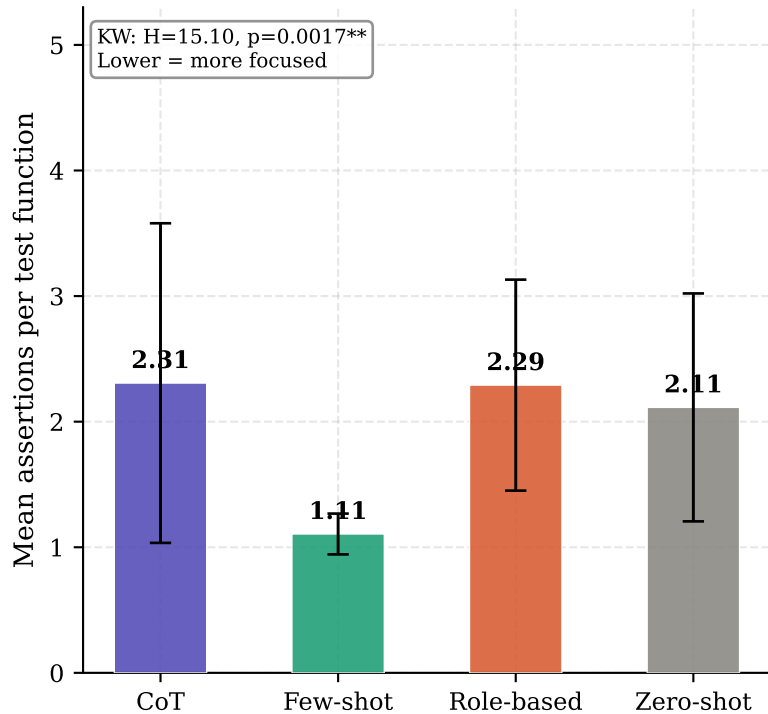
(b) Assertion density per test function
