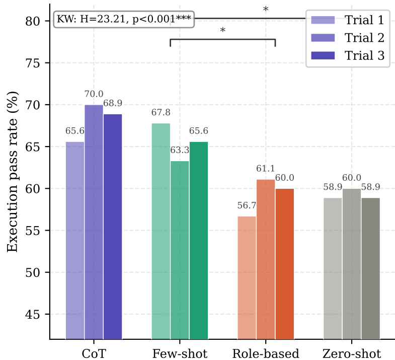
(a) Pass rate by strategy and trial
