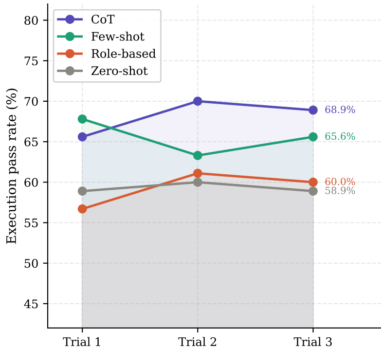
(b) Trial-to-trial stability
