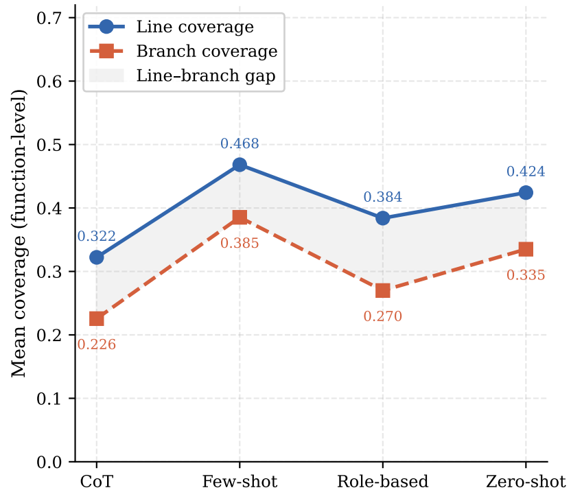
(b) Coverage gap between line and branch
