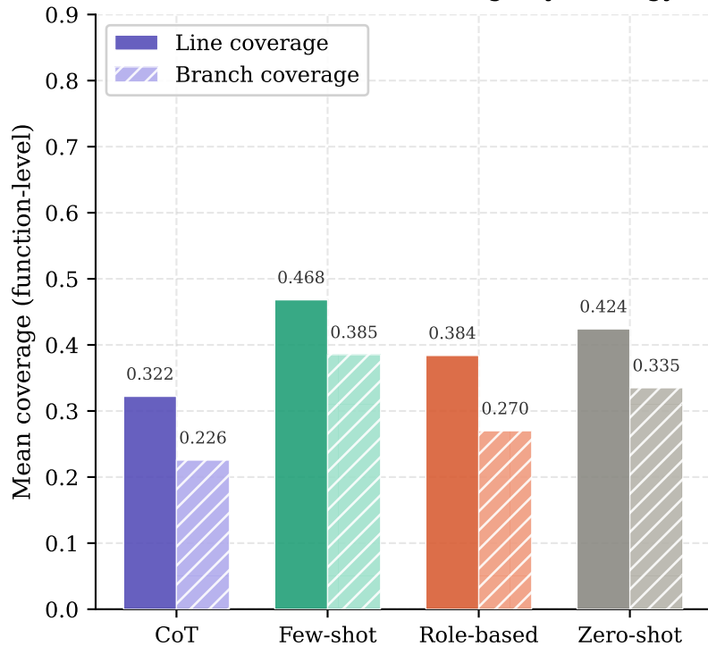
(a) Line and branch coverage by strategy
